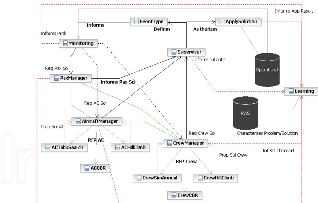
Fig. 5. MAS architecture
