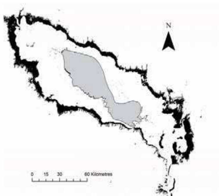
Fig. 7. Modelled reduction in flooded area from MODIS derived flood extents, with change shown in black.
