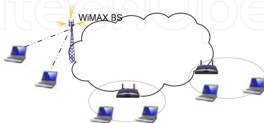
Fig. 7. Integrated WiMAX/WiFi wireless access.
