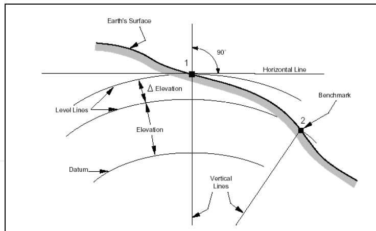
Fig. 1. Basic concept of topometric vertical control
