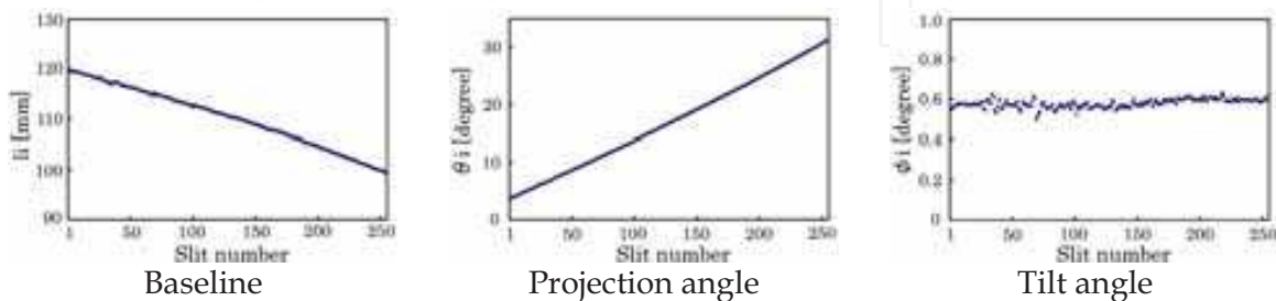
Fig. 6. Projector parameters.
