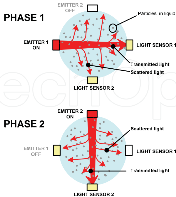
Fig. 2. Operation of four beam turbidimeter: light emission is alternated between emitters 1 and 2. During Phase 1, emitter 1 is on, sensor 1 receives the transmitted light, and sensor 2 receives scattered light; during Phase 2, the light emission is provided by emitter 2, transmitted light is received by light sensor 2, and scattered light, by light sensor 1.
