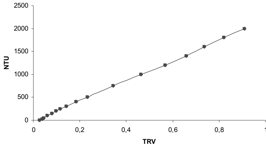
Fig. 13. Calibration curve obtained from the Turbidity Ratiometric Value (TRV). The appearance of the curve is much more linear than that of Fig. 11.
