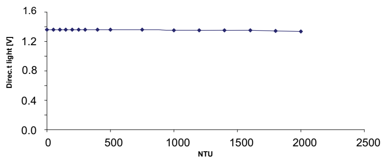
Fig. 9. Direct light as regards turbidity. Maximum variation is 1.5% over the turbidity span.
