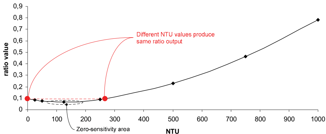
Fig. 5. The direct ratiometric measurement causes a no-defined problem due to the fact that different turbidity values produce the same output value. For example, a value is obtained with 260 NTU similar to that obtained with 0 NTU, which is completely unacceptable.
