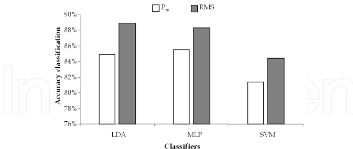
Fig. 9. Accuracy classification on motor-imagery dataset using standard periodogram for three proposed classifiers.
