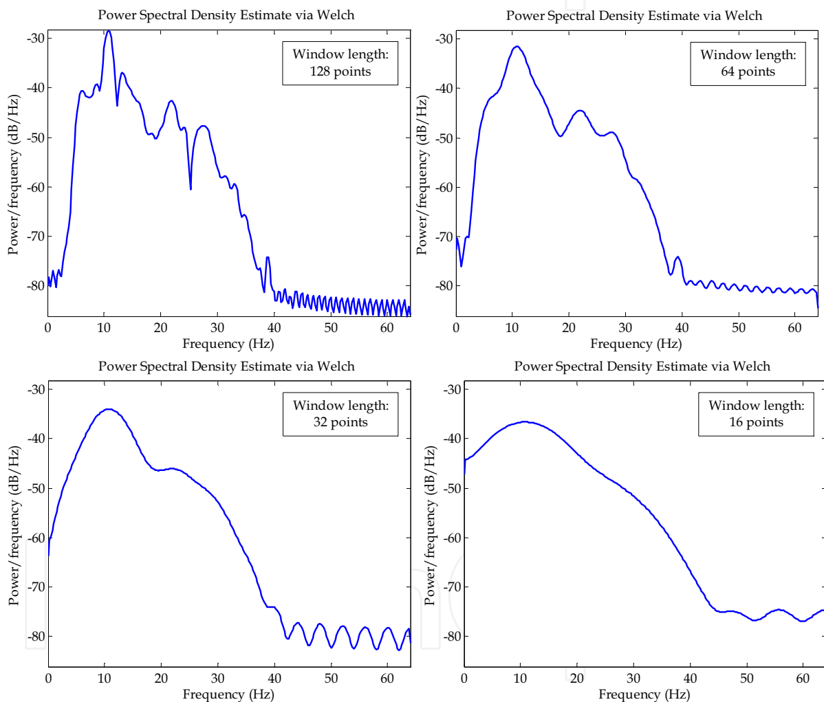
Fig. 4. Welch periodogram computed with a 512 points FFT, for different window length (128, 64, 32 and 16 points), from Motor-Imagery database, trial n o 1, between 4 to 6 s; from channel 1 (over C 3 ). The periodogram is smoothed when decreasing the window length. A Hamming window was applied in all cases. The EEG signal was filtered between 6 to 30 Hz.
