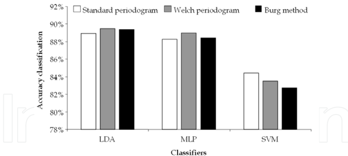
Fig. 14. Best accuracy classification obtained with each PSD estimation method proposed with the LDA, MLP and SVM.
