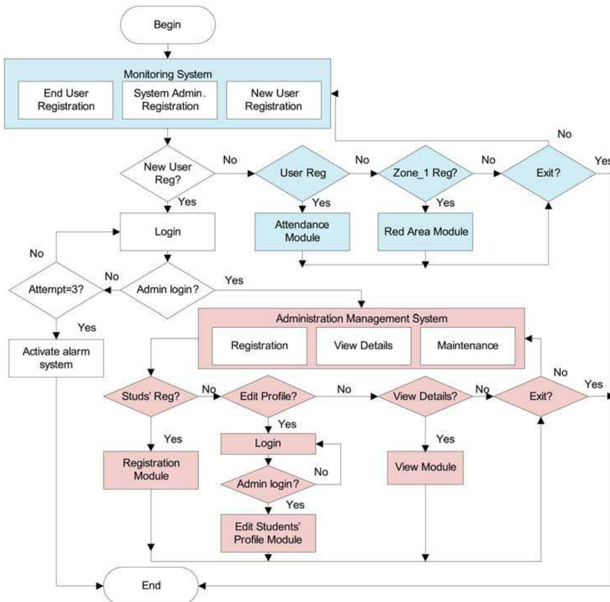
Fig. 4. Boarding school monitoring system flow
