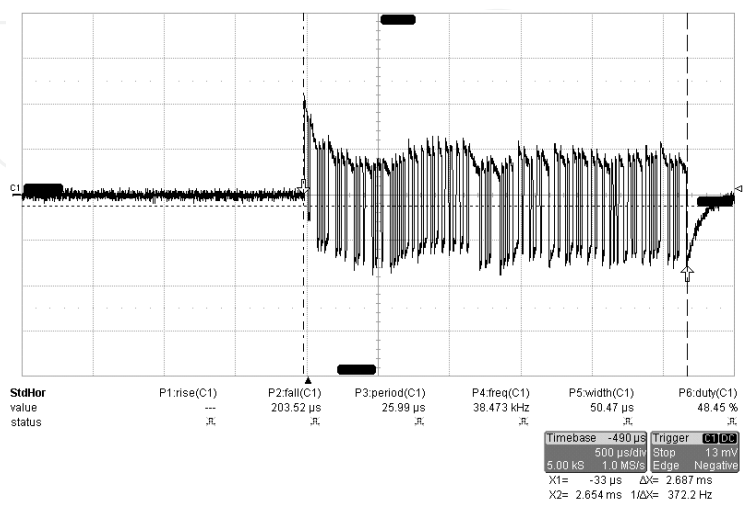
Fig. 4. Reading 1024 bits from one transponder takes 2.66 ms
