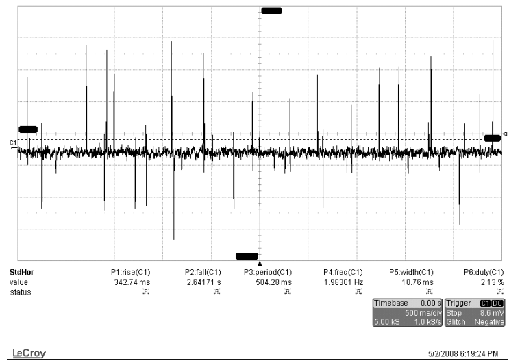
Fig. 3. Four transponders located in reader's range
