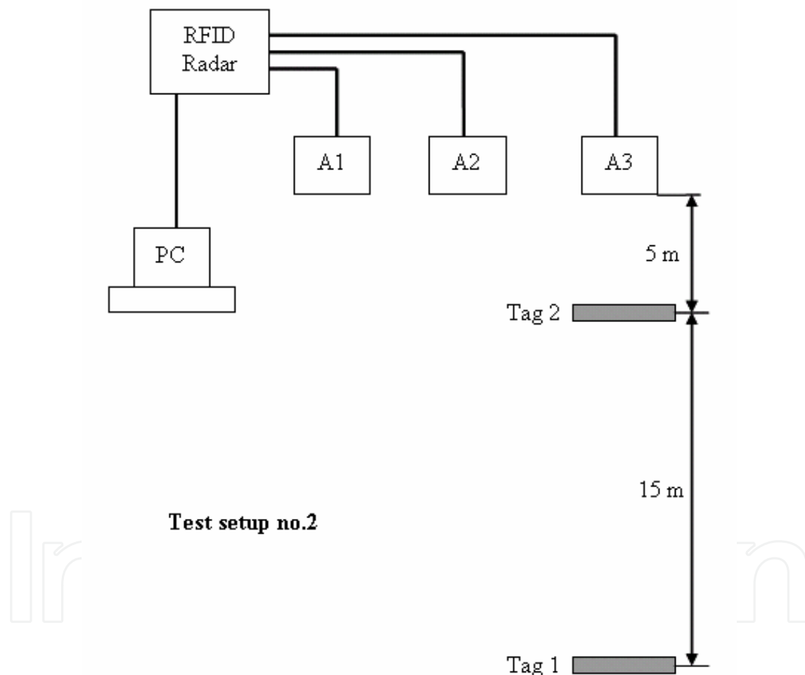
Fig. 9. Test setup for distance measurement for two tags - one at 5 m and the second at 20 m in front of the antenna
