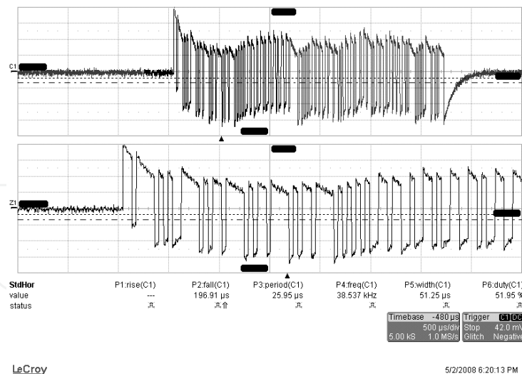
Fig. 5. Header data with one active transponder
