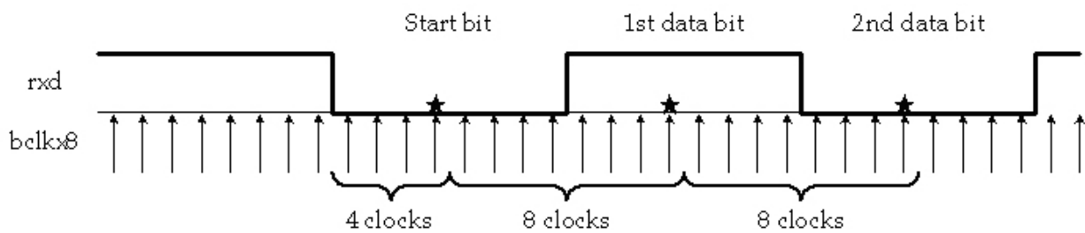
Fig. 4. Data sampling points by the UART receiver.
