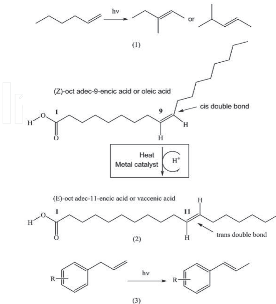
Figure 10. CCDB isomerization of straight chain alkenes (1), oleic acid (2) and Allyl benzene (3).
