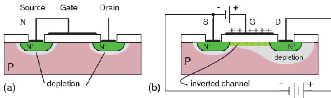
Figure 1. Schematic cross-section of a N-channel MOSFET: (a) 0 V gate bias, (b) positive gate bias that charges the gate. The P-type substrate below the gate takes on a negative charge. An inversion region with an excess of electrons forms below the gate oxide. This region connects the source and drain N-type regions, forming a continuous N-region from source to drain.
