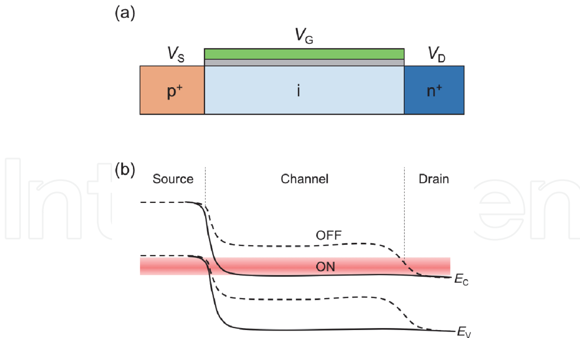
Figure 3. (a) Schematic cross-section of n-type TFET with applied source ( V_S ), gate ( V_G ) and drain ( V_D ) voltages. (b) Schematic energy band profile for the off-state (dashed lines) and the on-state (solid lines) in a n-type TFET.
