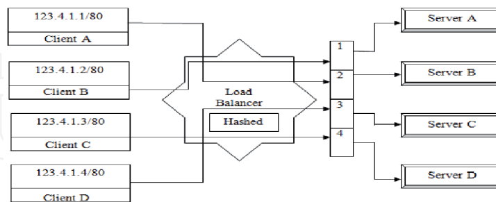
Figure 4. Stateless static load balancing.
