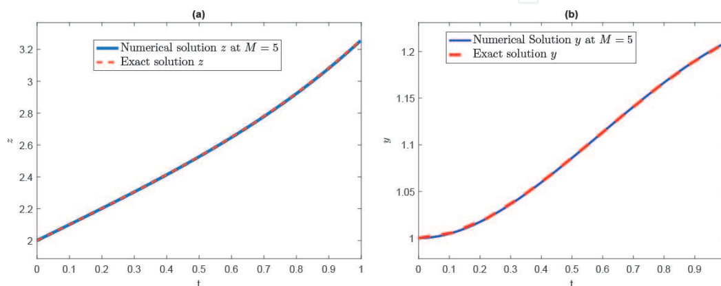
Figure 3. Plots of exact and approximate solution of Example 3.
