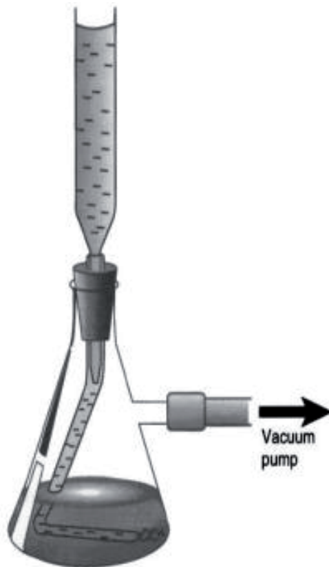
Figure 1. Experimental arrangement for concentration by forced dialysis [1].
