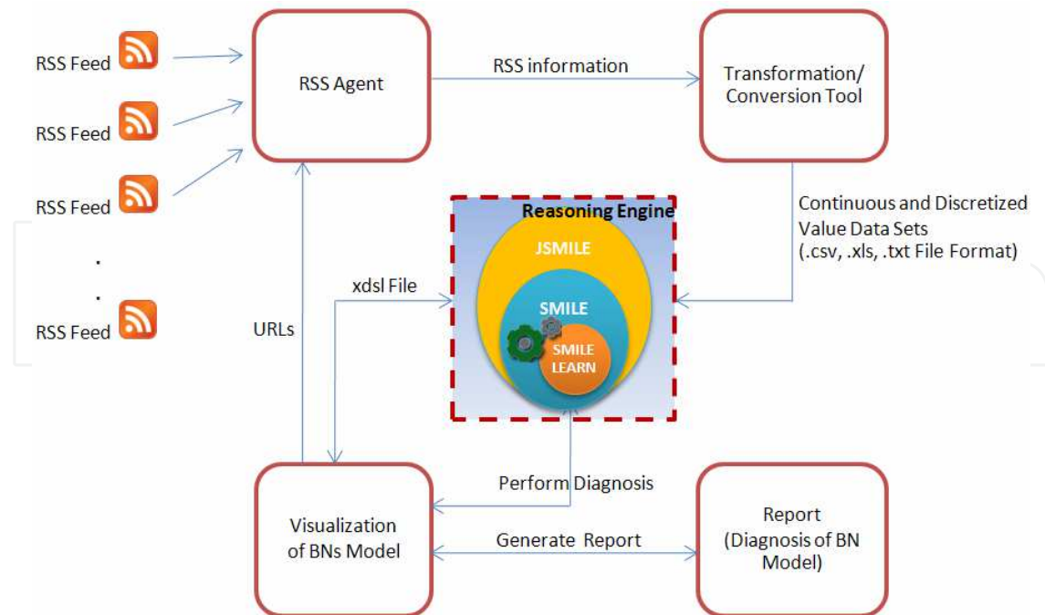
Fig. 1. A practical framework for automating the building of diagnostic BN models from online data sources
