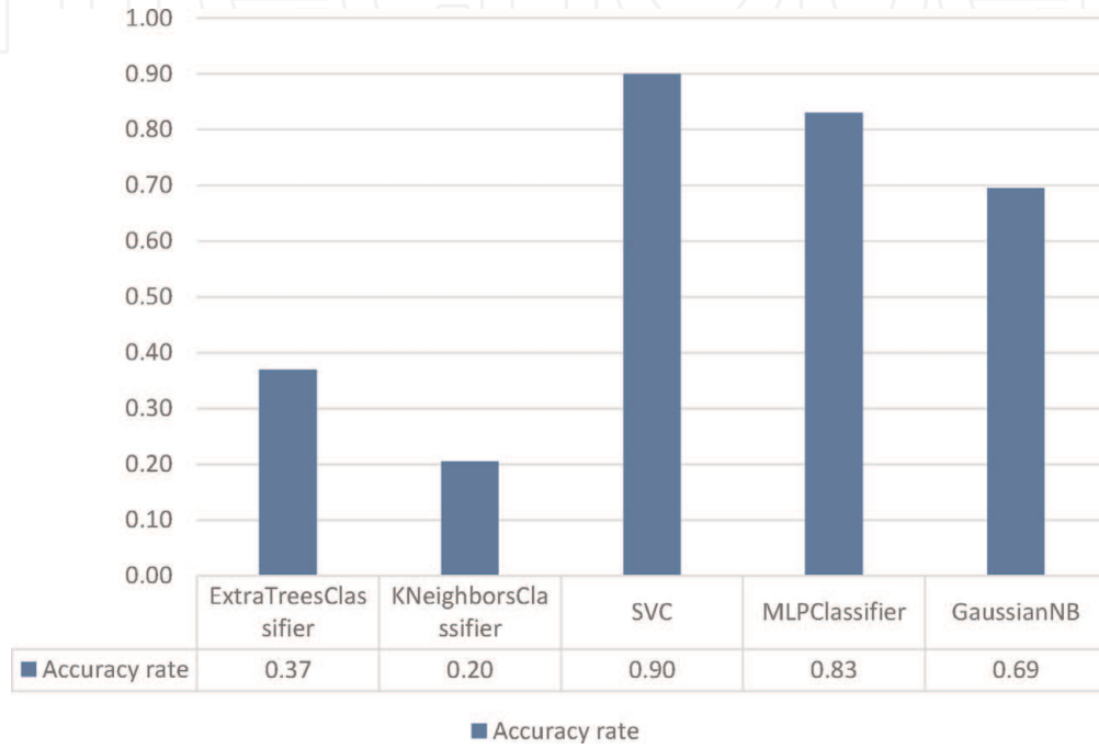
Figure 4. Classification accuracy on a data set.
