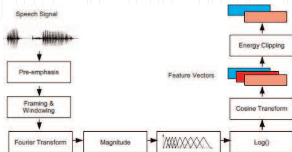
Figure 1. Steps involved in extracting MFCC feature vectors.
