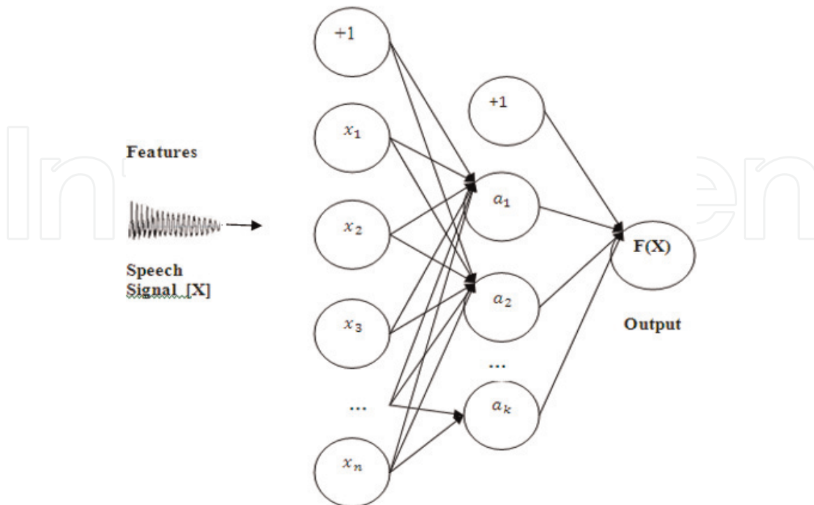
Figure 3. MLP architecture.
