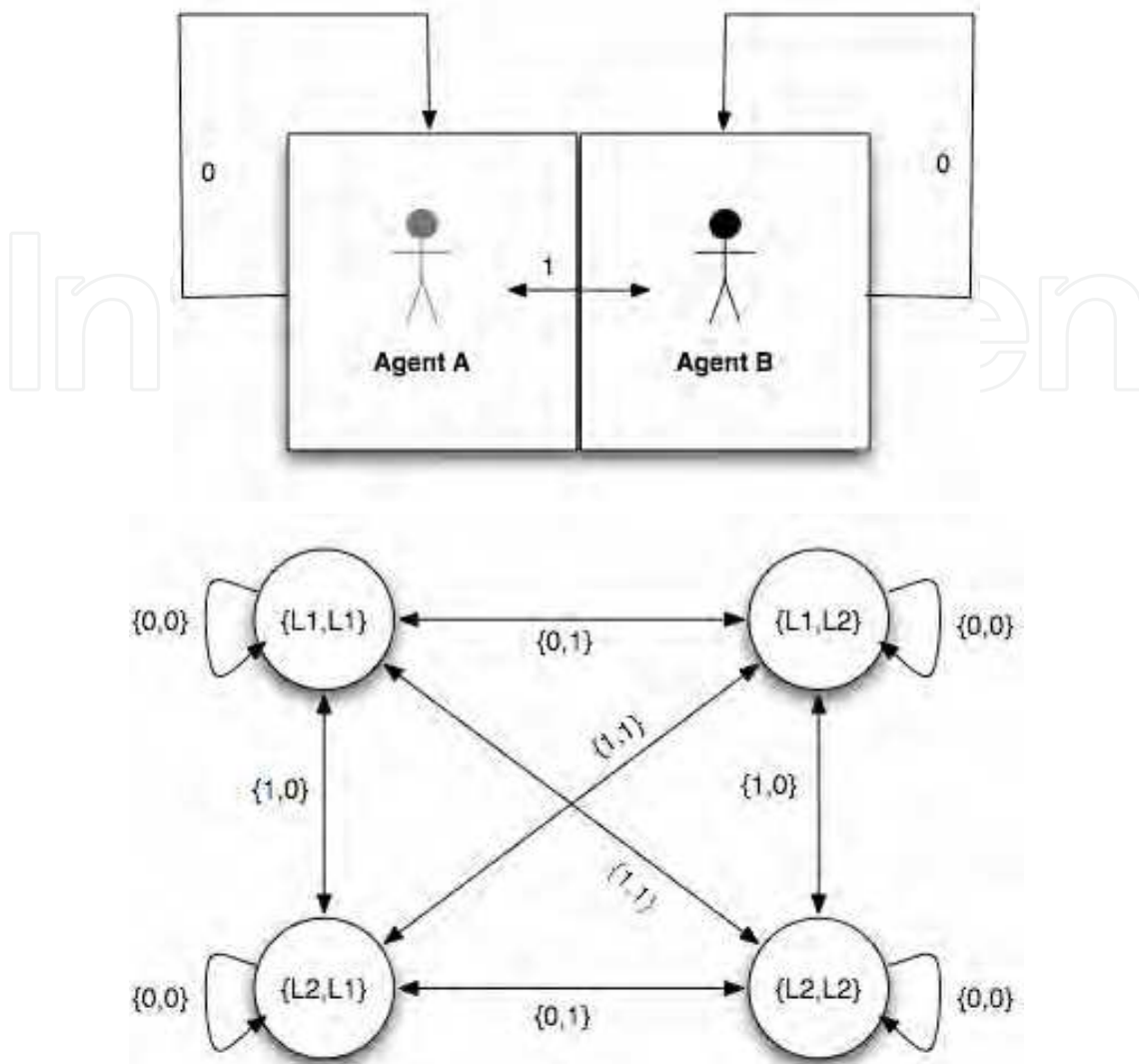
Fig. 3. A 2-location grid-world problem and its corresponding Markov game.
