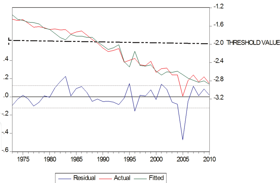
Figure 1. Actual, fitted and residual models.
