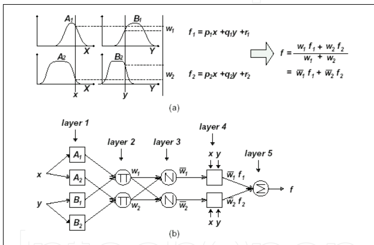
Fig. 5. ANFIS architecture
