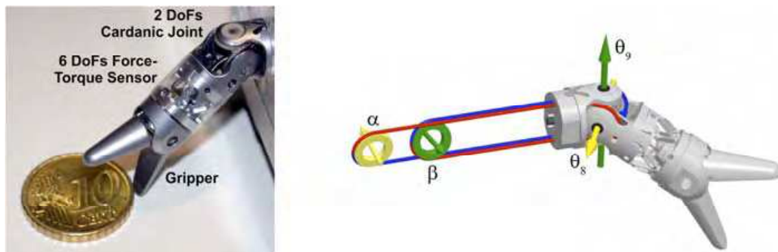
Figure 11. Prototype of instrument tip and layout of the drive cables
