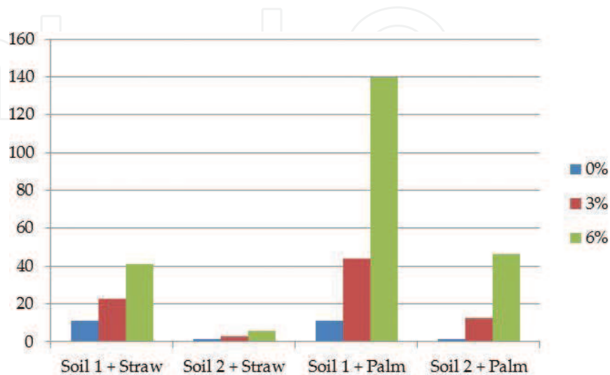
Figure 5. Saturated hydraulic conductivity (in cm/h) in soils amended with hay straw and palm tree leaves.
