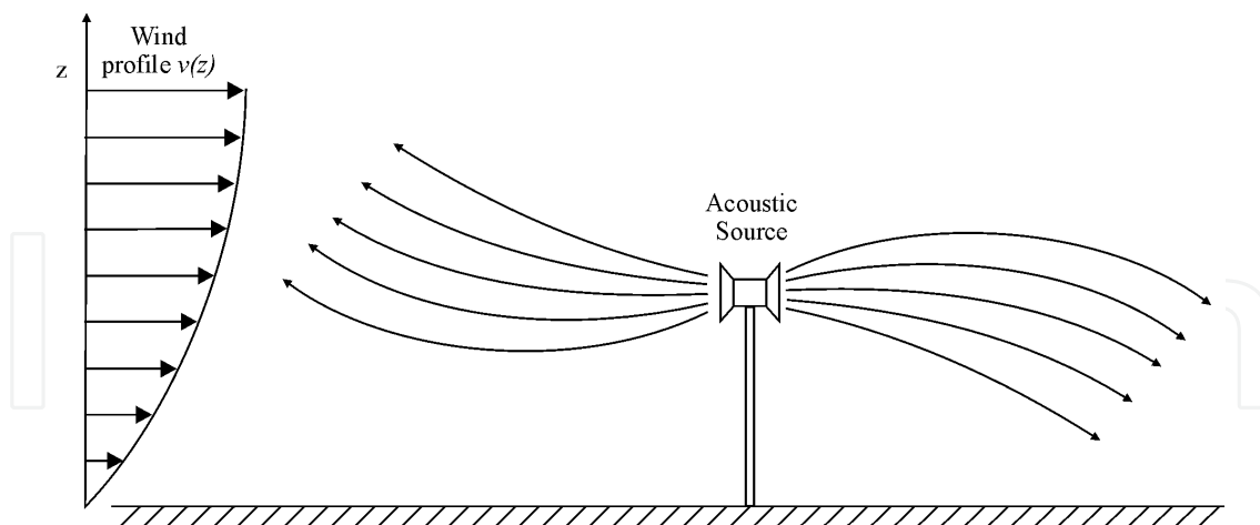
Fig. 4. Wind-induced refraction.
