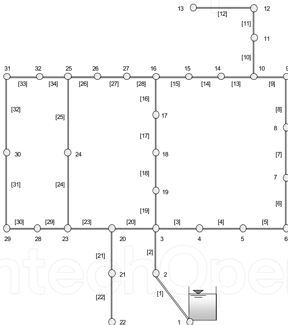
Figure 5. Network layout for the Hanoi Problem
