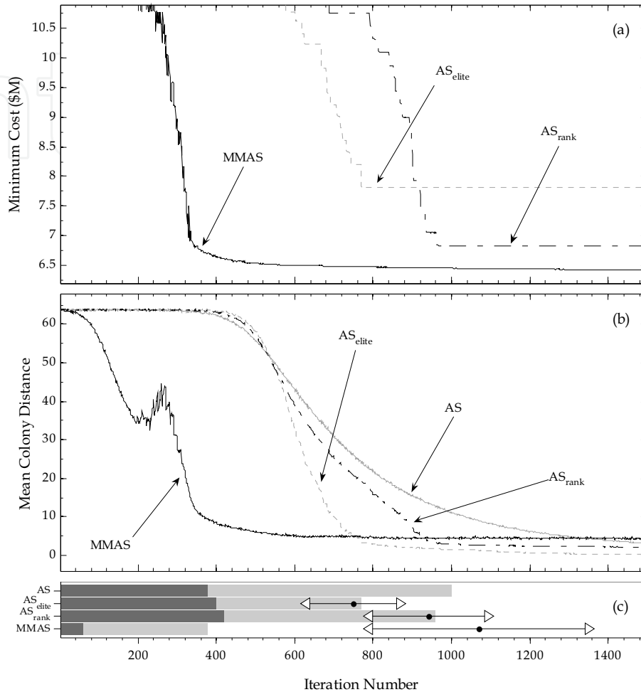
Figure 6. Plots of (a) the minimum cost ($M) found in each iteration f_{min}(t) , (b) the mean colony distance d_{\Sigma}(t) , and (c) run-time statistics for AS, AS_{elite} , AS_{rank} , and MMAS applied to the Hanoi Problem. Plots (a) and (b) are averaged from 20 runs. Plot (c) depicts the three convergence phases: phase-I (dark grey); phase-II (light grey); phase-III (remaining white space). The line graphs overlaying the bar charts in (c) indicate the search-time statistics (based on 20 runs) with the dot indicating the mean search-time, and the left and right arrows indicating the mean minus and plus a standard deviation, respectively
