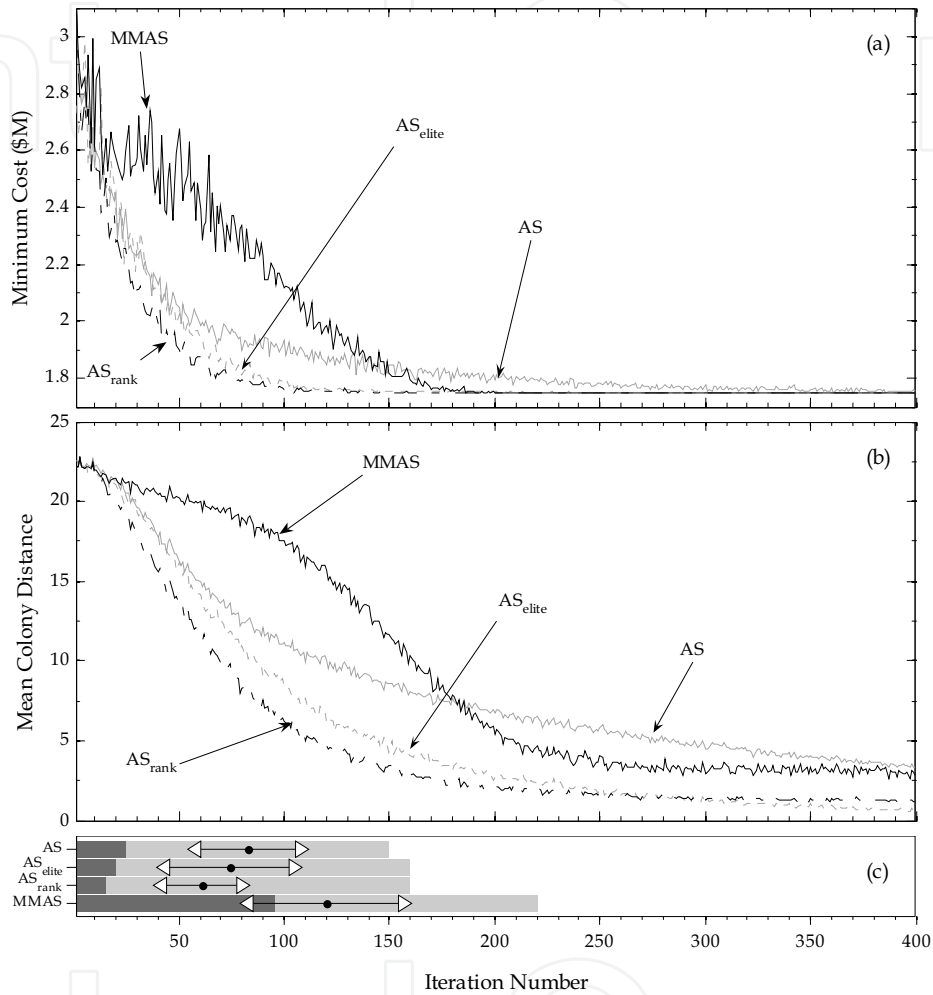
Figure 2. Plots of (a) the minimum cost ($M) found in each iteration f_{min}(t) , (b) the mean colony distance d_{\Sigma}(t) , and (c) run-time statistics for AS, AS elite , AS rank , and MMAS applied to the Two Reservoir Problem. Plots (a) and (b) are averaged from 20 runs. Plot (c) depicts the three convergence phases: phase-I (dark grey); phase-II (light grey); phase-III (remaining white space). The line graphs overlaying the bar charts in (c) indicate the search-time statistics (based on 20 runs) with the dot indicating the mean search-time, and the left and right arrows indicating the mean minus and plus a standard deviation, respectively.
