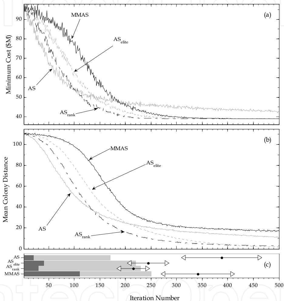
Figure 4. Plots of (a) the minimum cost ($M) found in each iteration f_{min}(t) , (b) the mean colony distance d_{\Sigma}(t) , and (c) run-time statistics for AS, AS elite , AS rank , and MMAS applied to the New York Tunnels Problem. Plots (a) and (b) are averaged from 20 runs. Plot (c) depicts the three convergence phases: phase-I (dark grey); phase-II (light grey); phase-III (remaining white space). The line graphs overlaying the bar charts in (c) indicate the search-time statistics (based on 20 runs) with the dot indicating the mean search-time, and the left and right arrows indicating the mean minus and plus a standard deviation, respectively
