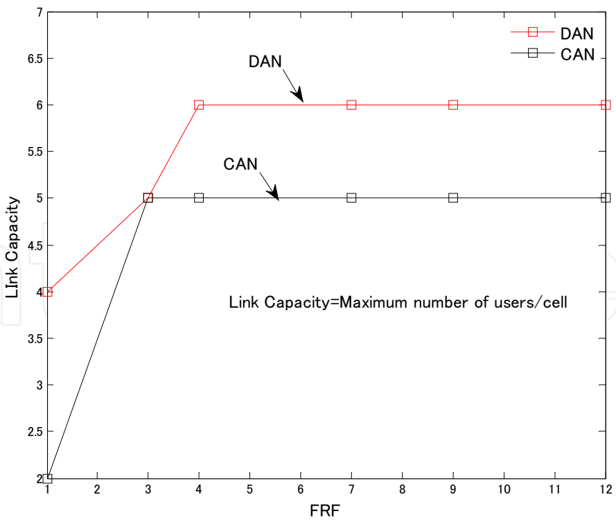
Figure 10. Link capacity.
