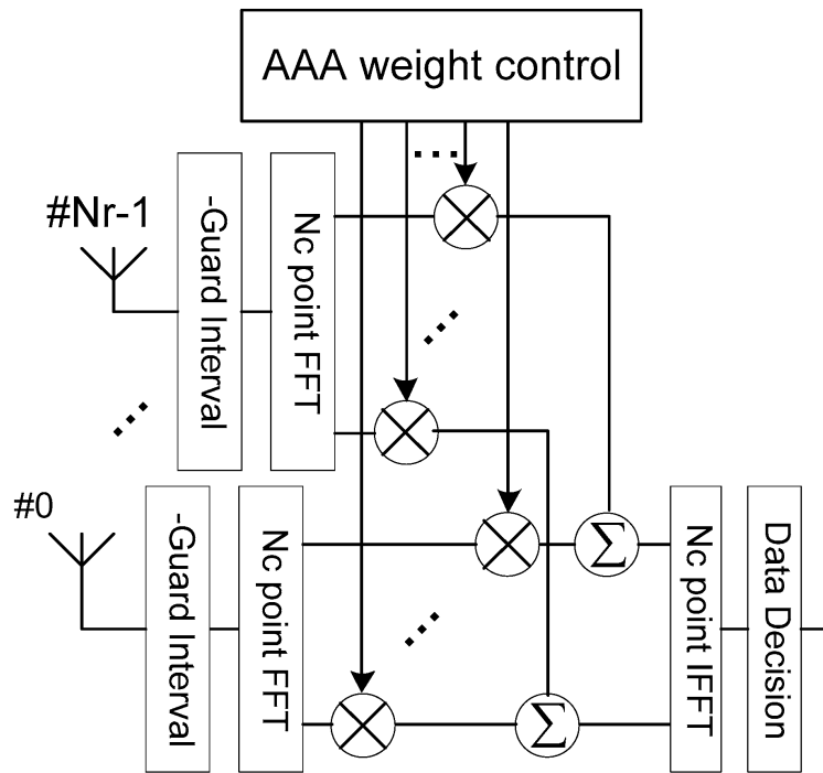
(b) Receiver
