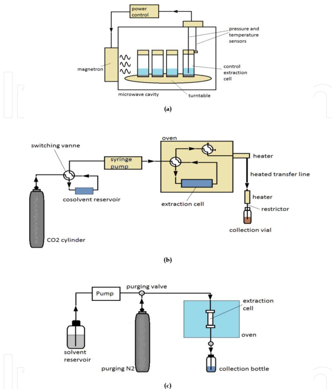
Figure 2. Extraction apparatus (a) Microwave-Assisted Extraction: MAE extraction vessels are placed on a turntable inside an oven and are subjected to microwave irradiations generated by a magnetron. A programmable microcomputer controls and monitors the power, temperature and pressure within the vessel (b) Supercritical Fluid Extraction: SFE incorporates pumps which produce the high pressures required for supercritical CO 2 work. An organic cosolvent can be added to the extraction fluid by a separate module. The extraction cell is placed in an oven which maintains a precise fluid temperature. A static mode (equilibration) and a dynamic mode (with a controlled flow-rate) can be performed successively. A restrictor valve (changing the CO 2 from condensed to gaseous phase) provides precise control over flow-rates (c) Assisted-Solvent Extraction: ASE operates by moving the extraction solvent through an extraction cell which is heated by direct contact of the oven. Extractions can be performed first in static mode; when the extraction is complete, compressed nitrogen moves the heated extracting solvent to the collection bottle.
