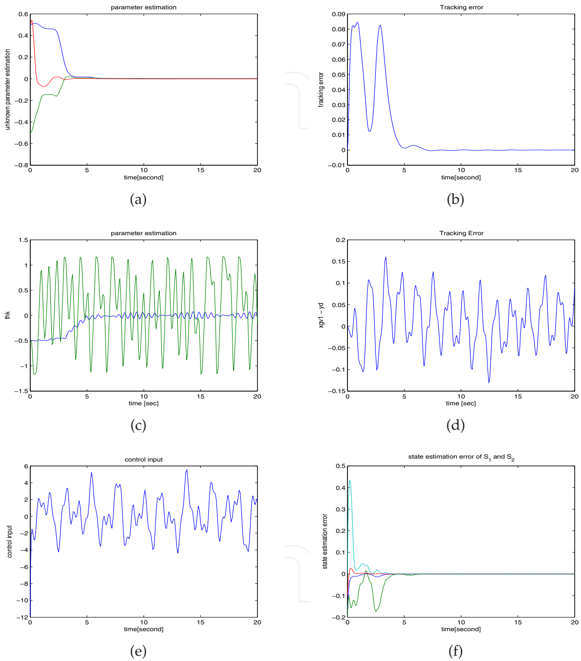
Figure 2. System response for Example under command input d(t) = 0.4 \sin(0.1t) + \sin(0.6t) , \dot{w}_1 = 0 , \dot{w}_2 = 0 , \dot{w}_3 = 0 , \check{w}_1(t) = \sin(12t + \frac{\pi}{9}) + 0.8 \sin(3t) , and \check{w}_2(t) = 3 \sin(3t + \frac{\pi}{3}) . (a) Parameter estimate; (b) Tracking error; (c) Parameter estimate(based on [17]); (d) Tracking error(based on [17]); (e) control input; (f) State estimation error;
