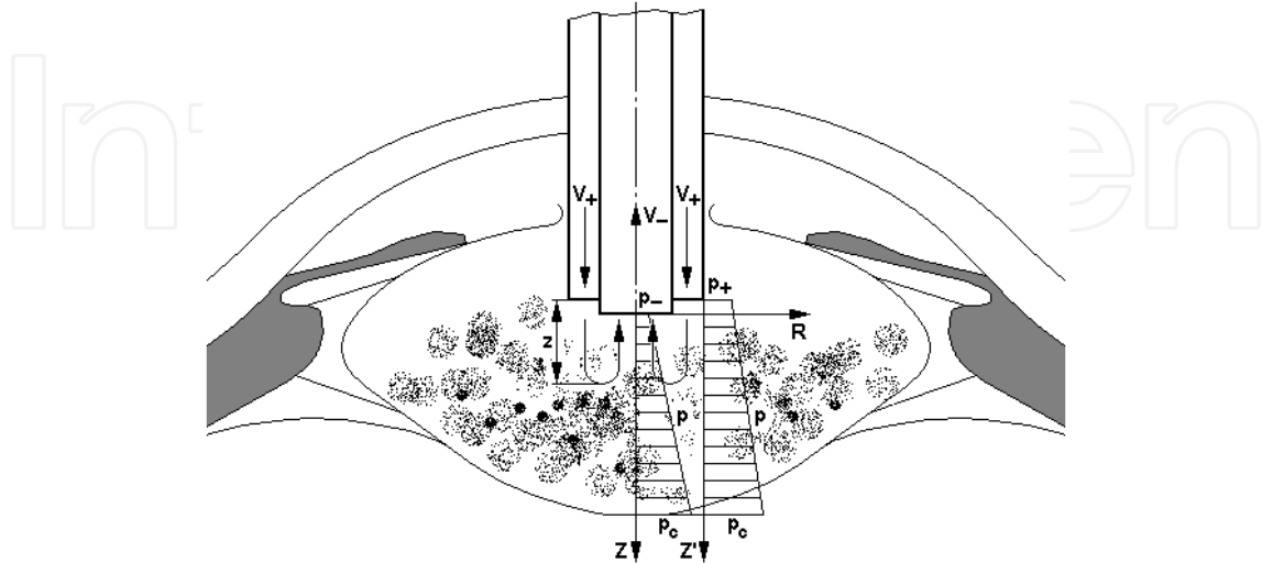
Fig. 3. Pressure distribution ( p ) and displacement of fluid particles ( z ) in the coaxial technique
