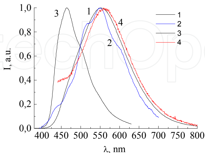
Figure 5. Spectra of \text{Zn}(\text{DFP-SAMQ})_2 based devices: EL spectra of the devices D10 ITO/PTA/NPD/ \text{Zn}(\text{DFP-SAMQ})_2/\text{AlCa} (1) and D11 ITO/PTA/ \text{Zn}(\text{DFP-SAMQ})_2/\text{AlCa} (2); PL spectra of \text{Zn}(\text{DFP-SAMQ})_2 powder (3) and of PTA: \text{Zn}(\text{DFP-SAMQ})_2 mixed film (4).
