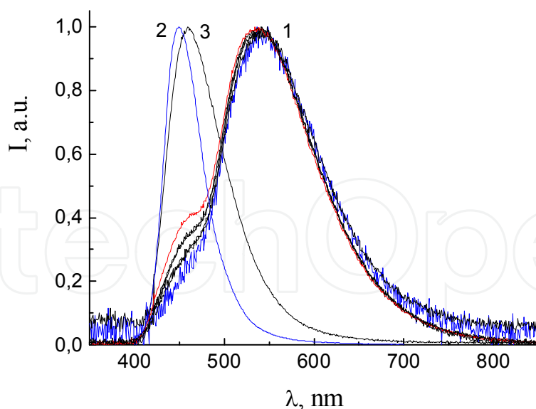
Figure 4. Spectra of \text{Zn}(\text{POPS-BTZ})_2 based devices: Normalized EL spectra of the device D8 ITO/PTA/NPD/ \text{Zn}(\text{POPS-BTZ})_2/\text{Al:Ca} for bias voltages 4.0 V (blue curve), 4.5, 5.0, 5.5 V (black curves) and 6.0 V (red curve) (1), PL of \text{Zn}(\text{POPS-BTZ})_2 powder (2) and the EL spectrum of the device D9 ITO/PTA/NPD/CBP/ \text{Zn}(\text{POPS-BTZ})_2/\text{Al:Ca} (3)
