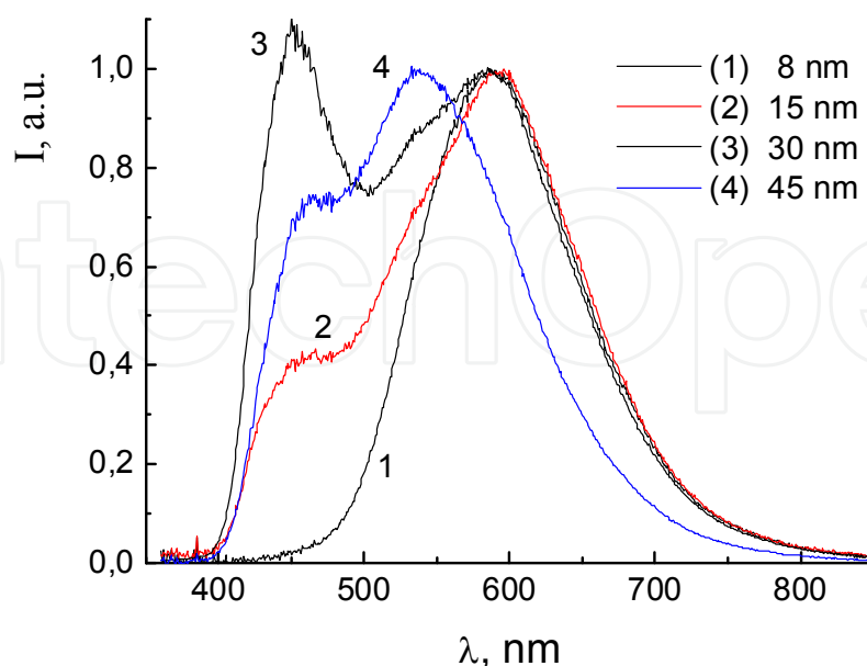
Figure 6. Normalized EL spectra of ITO/PTA/NPD/ Zn(TSA-BTZ)_2 /Al:Ca devices with different thicknesses of NPD layer: 8 nm (1), 15nm (2), 30 nm (3) and 45 nm (4). Spectra are measured at the same current 7.4 \text{ mA/cm}^2 for all devices.
