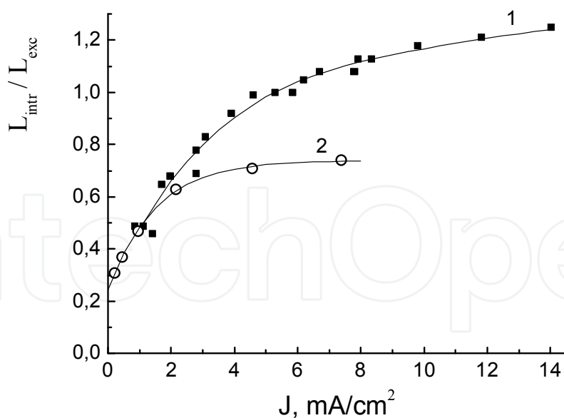
Figure 8. Plot of relative intensities of the intrinsic EL band and that of exciplex band as a function of the current for the devices ITO/PTA/NPD/ \text{Zn}(\text{TSA-BTZ})_2/\text{Al:Ca} with NPD layer thicknesses 30 nm (1, squares) and 45 nm (2, circles). Solid curves represent only guide to an eye.
