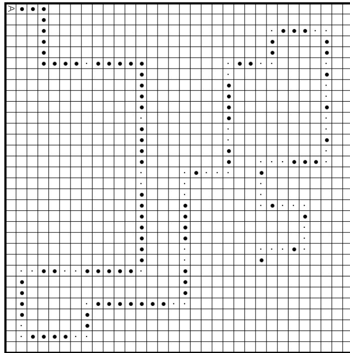
Figure 1. Illustration of the Santa Fe Trail (the ant starts in the upper left corner, heading to the east, large dots are food pellets, and small dots are empty cells on the ideal path).
