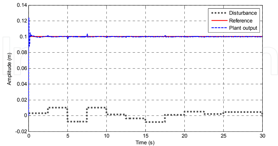
Figure 12. System response on step reference tracking, using only the robust controller, and in uniformly distributed white noise presence
