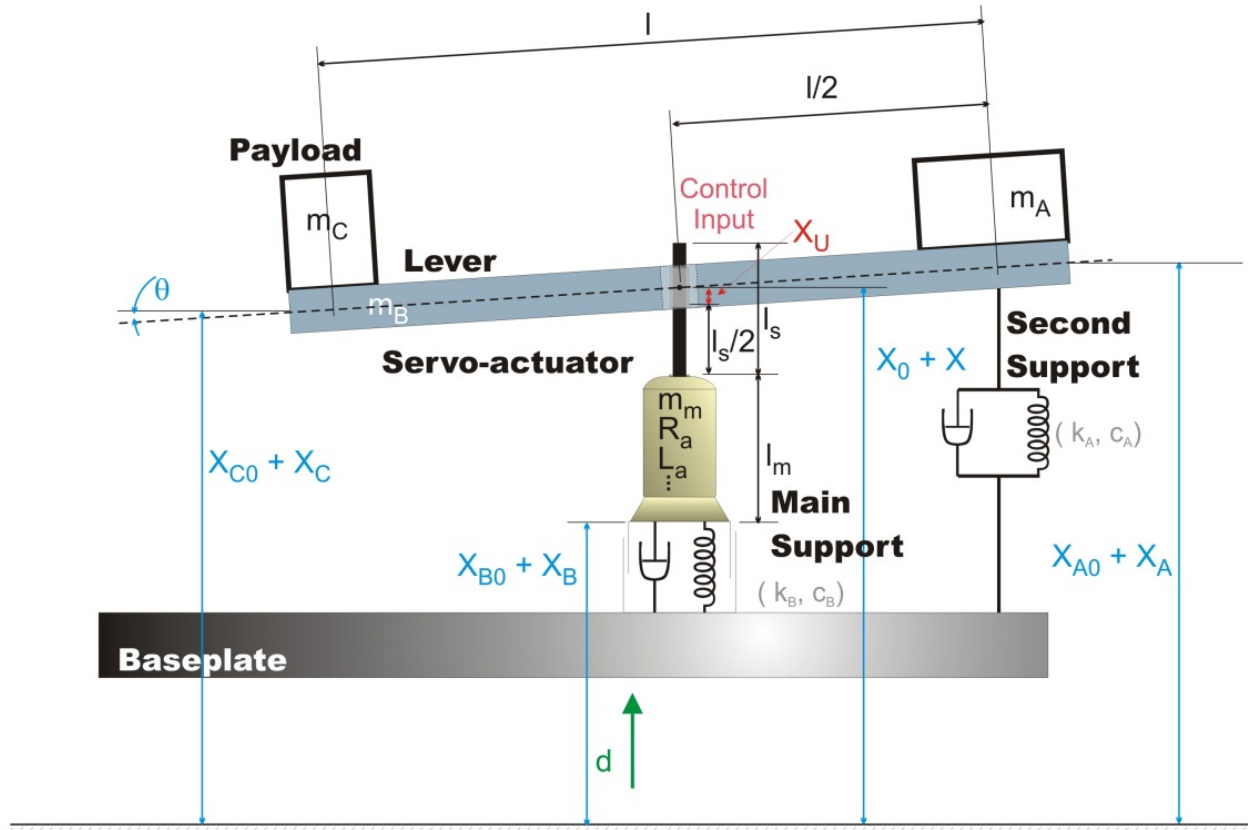
Figure 2. Electromechanical system
