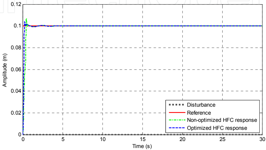
Figure 25. Comparison of the two hierarchical controllers in tracking a step reference
