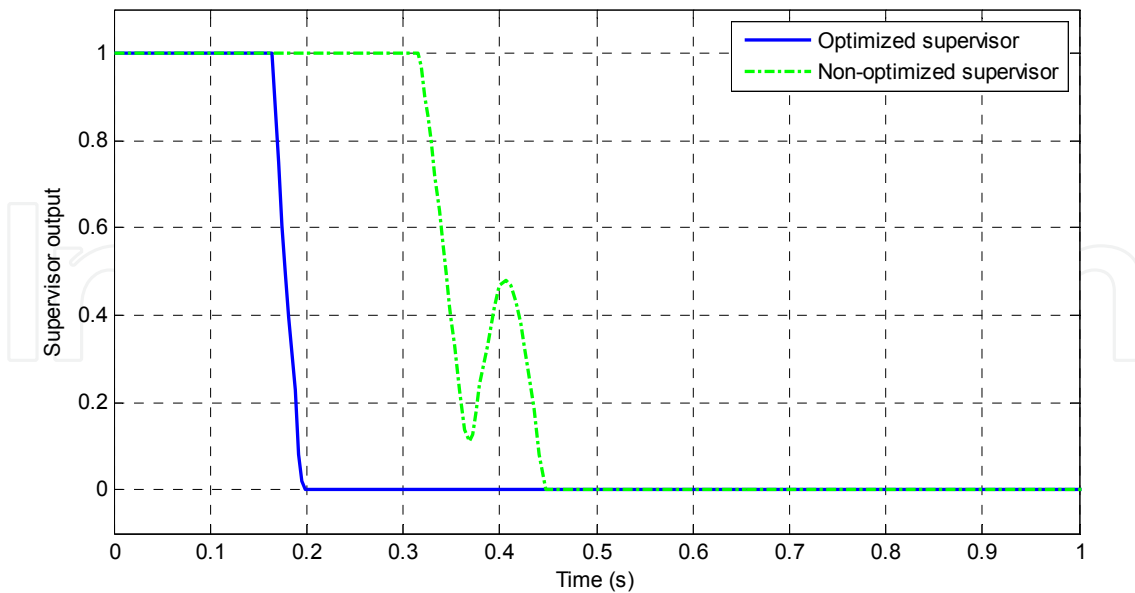
Figure 27. Comparison of signals generated by the two supervisors in tracking a step reference
