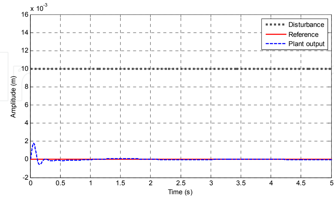
Figure 8. System response on step disturbance rejection, only with the robust controller, and with a null reference
