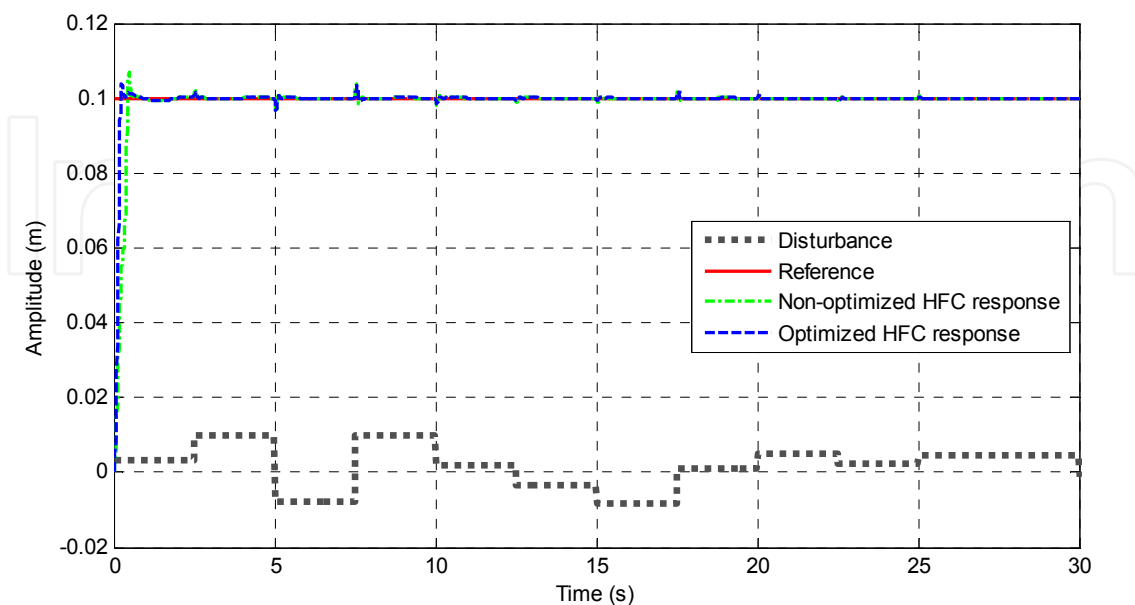
Figure 28. Comparison of the two HFC in tracking a step reference under disturbance
