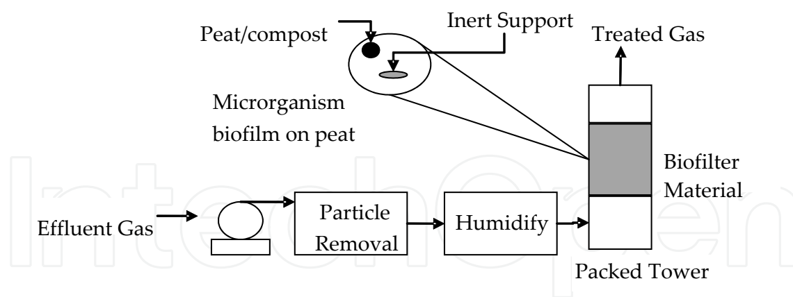
Figure 4. Illustrative depiction of a typical biofilter operation.
