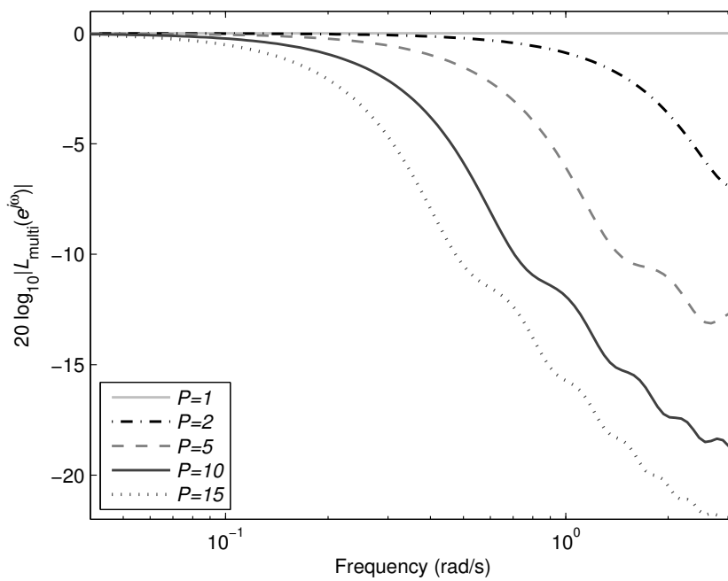
Fig. 2. Magnitude frequency response of L_{\text{multi}}(e^{j\omega}) for increasing prediction horizon length.
