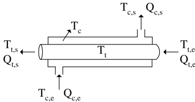
Fig. 3. Schematic heat exchanger.
