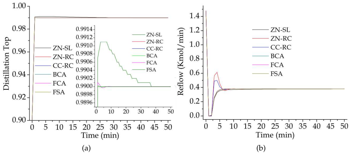
Fig. 2. Distillation top profile (a) and reflow profile (b) using classical and BiOM.
