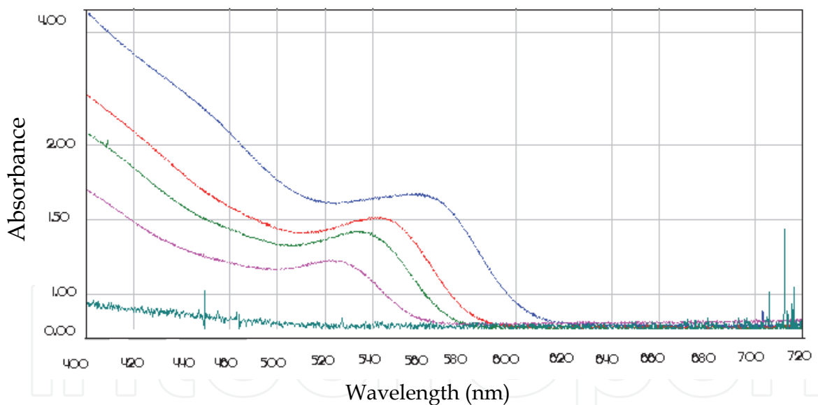
Fig. 4. UV-Vis spectra of Cd-Se colloidal suspension
