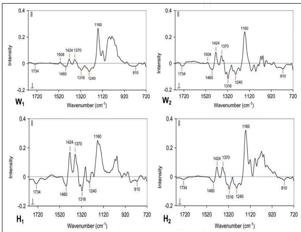
Fig. 18. Average orientation spectra of the two W fibres (W1 and W2) and the two H fibres (H1 and H2): cellulose 1160 cm -1 , 1316 cm -1 , 1370 cm -1 and 1424 cm -1 , glucomannan 810 cm -1 , xylan 1734 cm -1 , 1460 cm -1 and 1240 cm -1 and lignin 1508 cm -1 [86]
