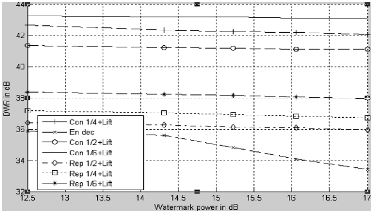
Fig. 13. DWR vs watermark power for direct embedding on entropy decoded data and using both channel coding and lifting
