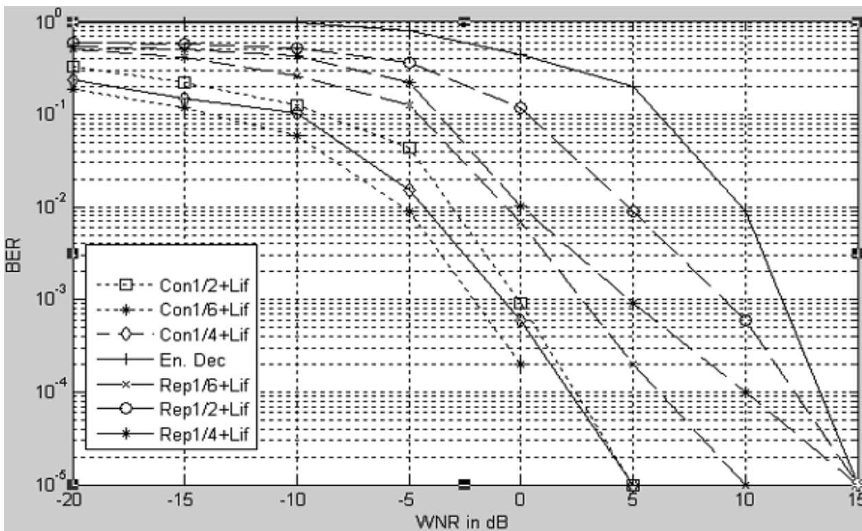
Fig. 14. BER performance at different watermark- to-noise (WNR) in dB
