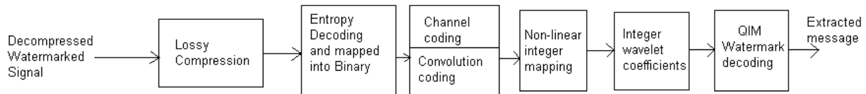
Fig. 3. Block diagram representation of watermark decoding scheme
