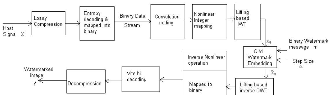
Fig. 2. Block diagram representation of watermark embedding scheme
