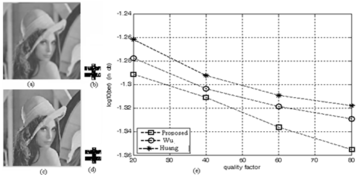
Fig. 15. (a), (c): Watermarked images after mean and median filtering, respectively, (b) and (d): Extracted watermarks from (a), and (c), respectively, (e) Robustness performance comparison against JPEG compression
