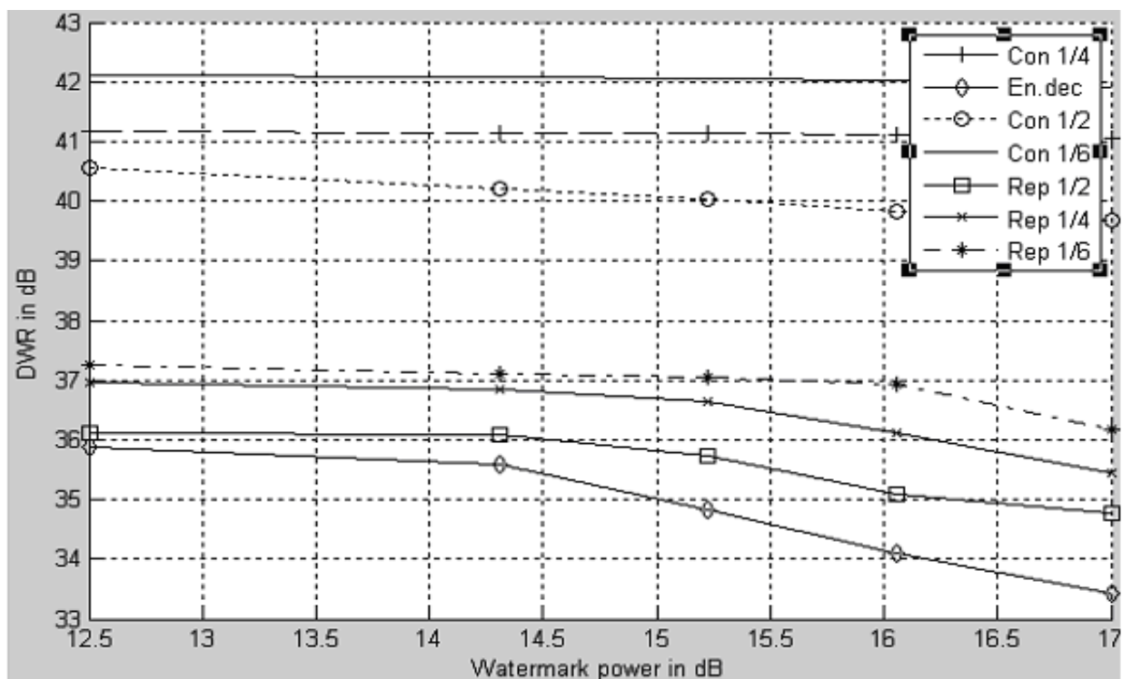
Fig. 12. DWR vs watermark power for direct embedding on entropy decoded data and using channel coding, namely convolution coding and repetition coding
