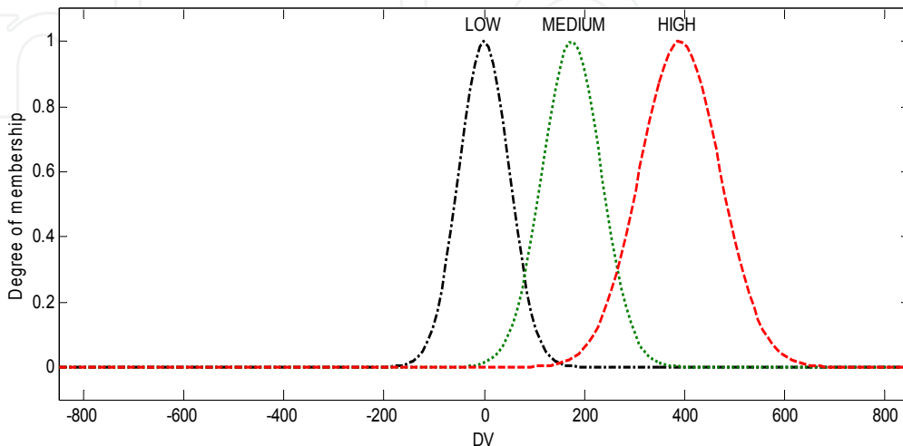
Fig. 8. Membership function for input 2 (DV)
