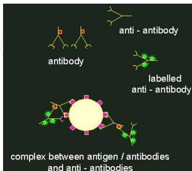
Fig. 11. Depicting antigen-antibody complex
