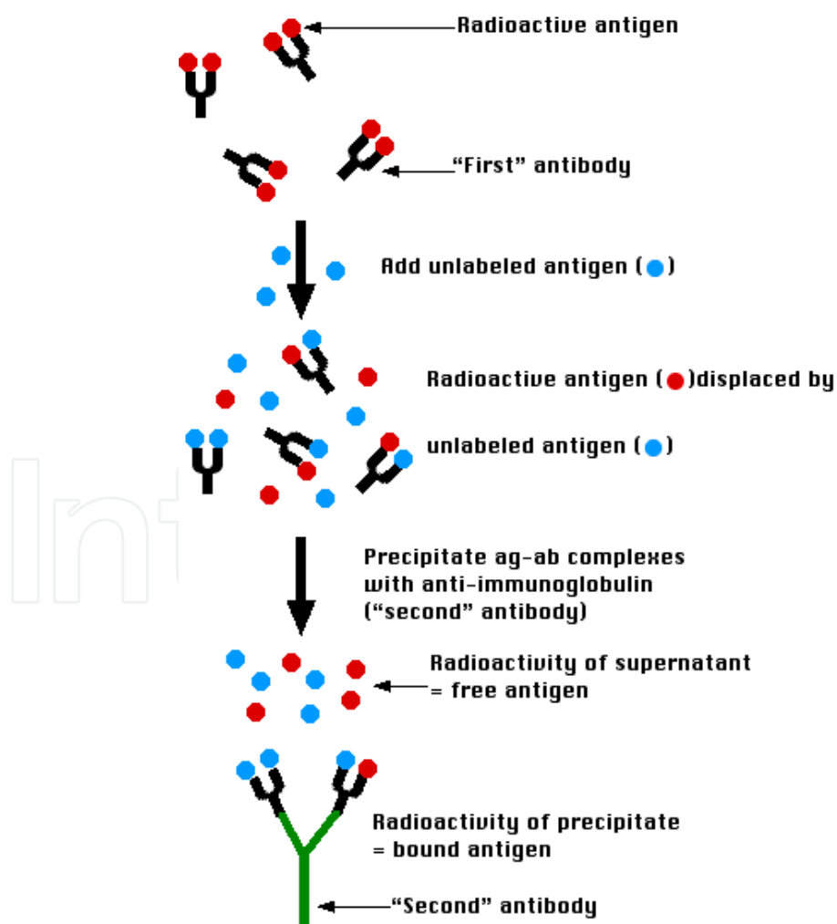
Fig. 12. Flow diagram of the process of radioimmunoassay.
