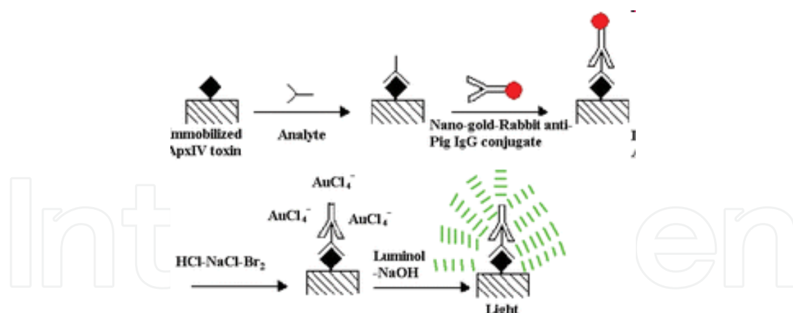
Fig. 9. Schematic diagram of chemi-luminescent Immunoassay.
