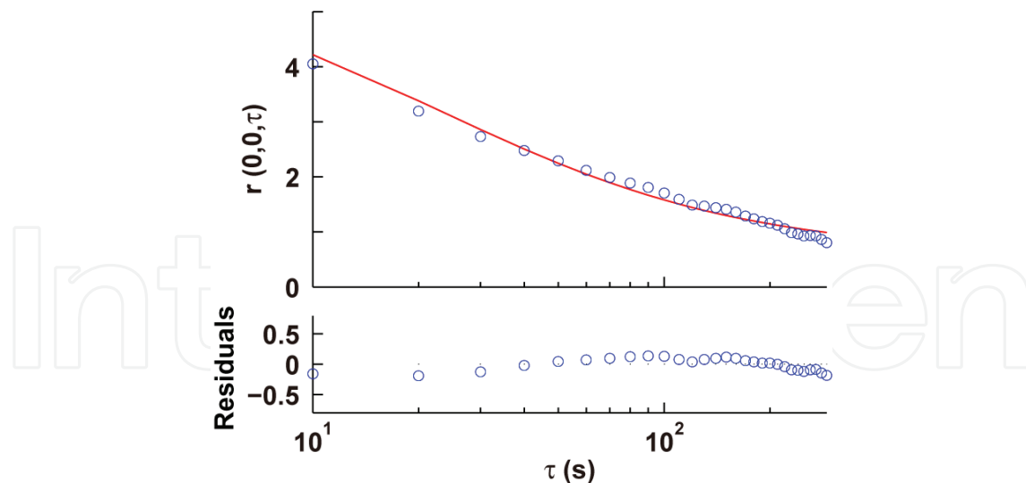
Fig. 6. Typical dynamics of mtDNA analyzed by ICS. In upper panel, temporal image correlation function of raw data (open circles) and fitted analytical model (solid line) are shown. Lower panel is the residuals.
