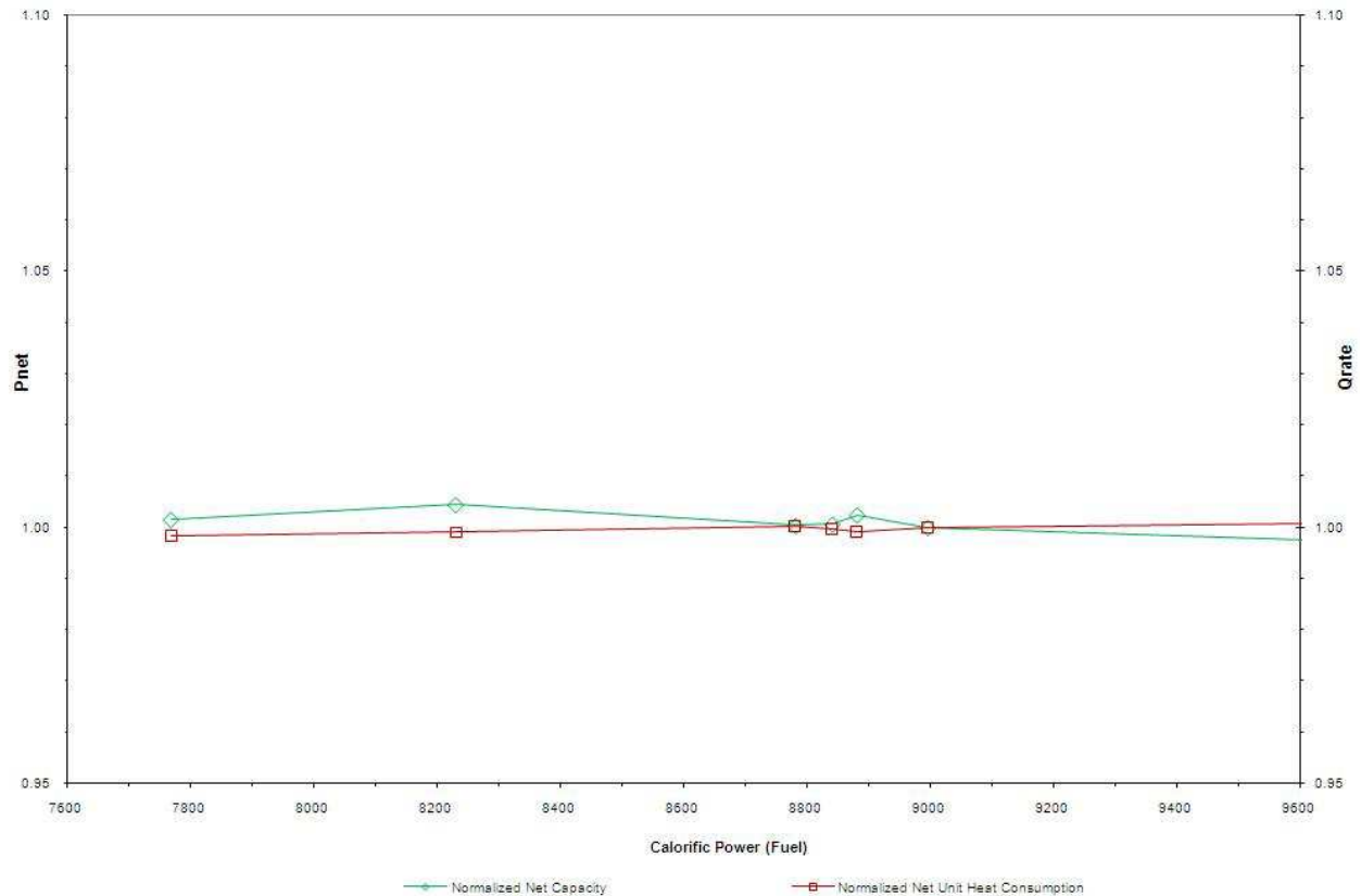
Fig. 6. Correction curve by calorific value of fuel.
