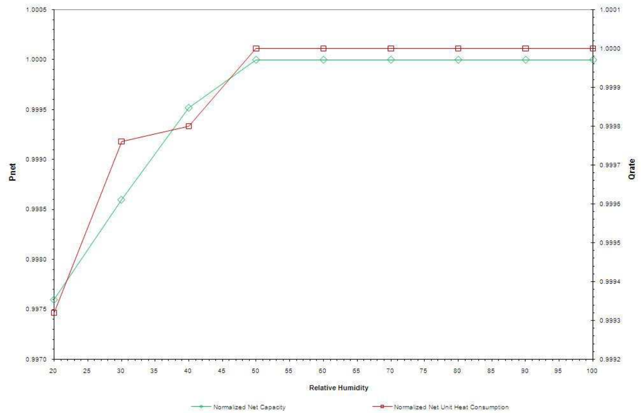
Fig. 5. Correction curve by humidity.
