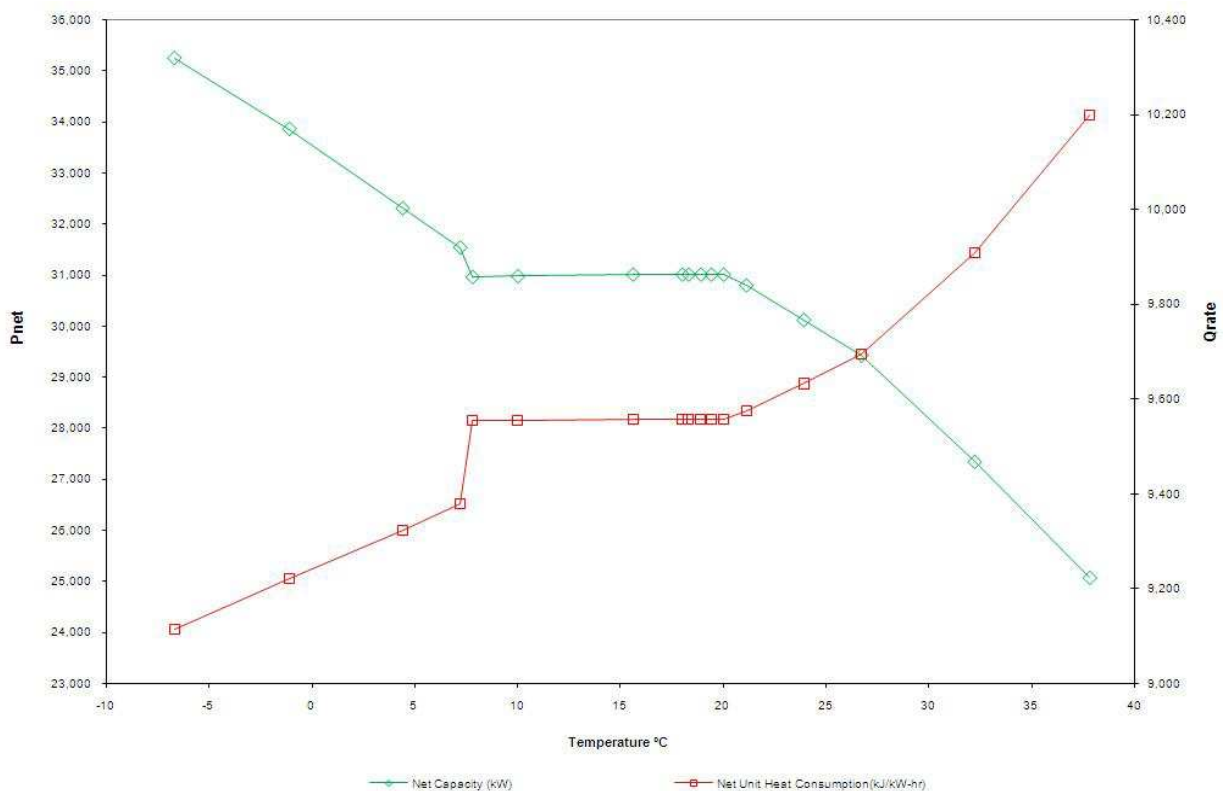
Fig. 3. Correction curve by temperature.
