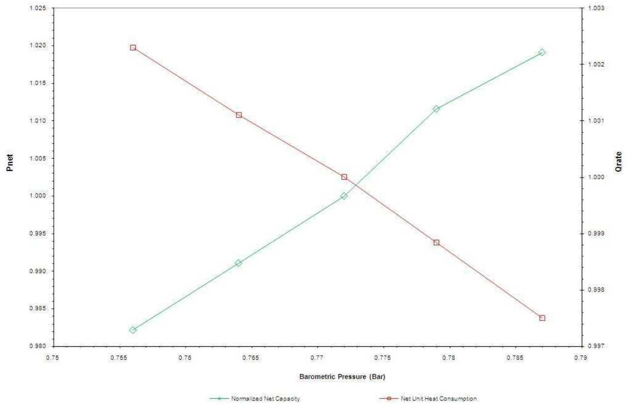
Fig. 4. Correction curve by barometric pressure.
