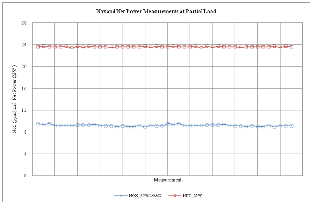
Fig. 8. NO x measurements (ppm) and Net Power (MW) recorded during test at 75% load.
