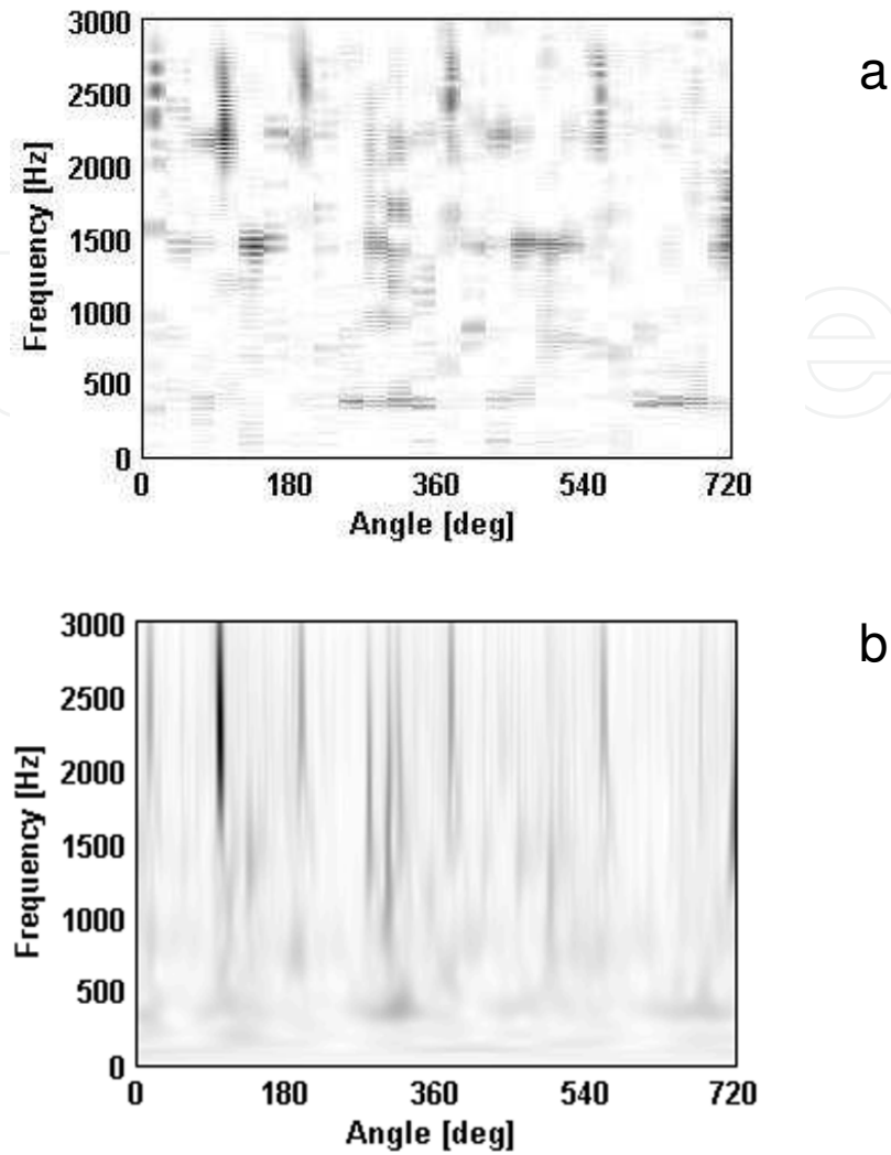
Fig. 9. Faulty engine – (a) CWT of the TSA: purification method (impulse mother wavelet); (b) TDAS method (morlet mother wavelet).
