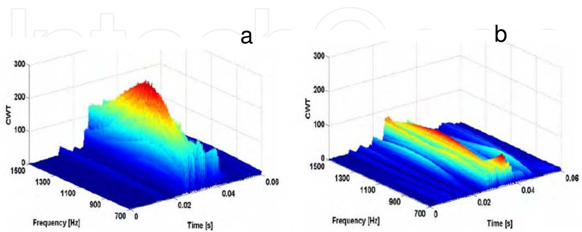
Fig. 6. Continuous wavelet transform (Morlet wavelet) for transom left-side acceleration, 700-1500 Hz frequency range; Coupling: Type 1 (a) and Type 2 (b).
