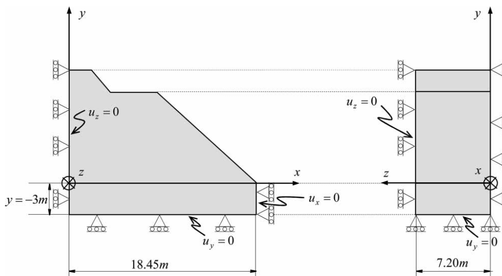
Fig. 7. Boundary conditions
