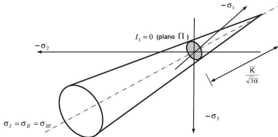
Fig. 8. Schematic of yield surfaces Drucker-Prager
