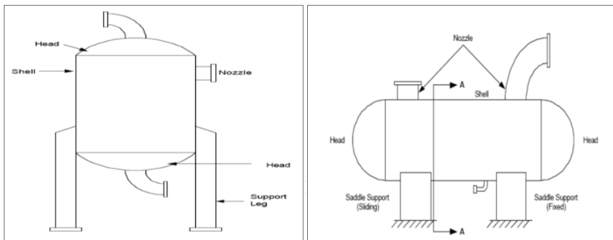
Subfigure 1: Typical horizontal vessel Source: Megyesy. E.F (2001)
