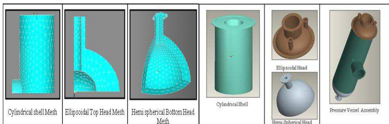
Subfigure 1: Design model for case one
