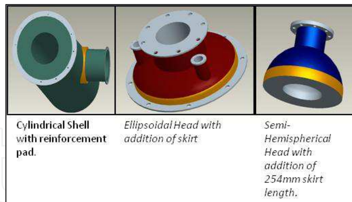
Fig. 4. Design model for case three
