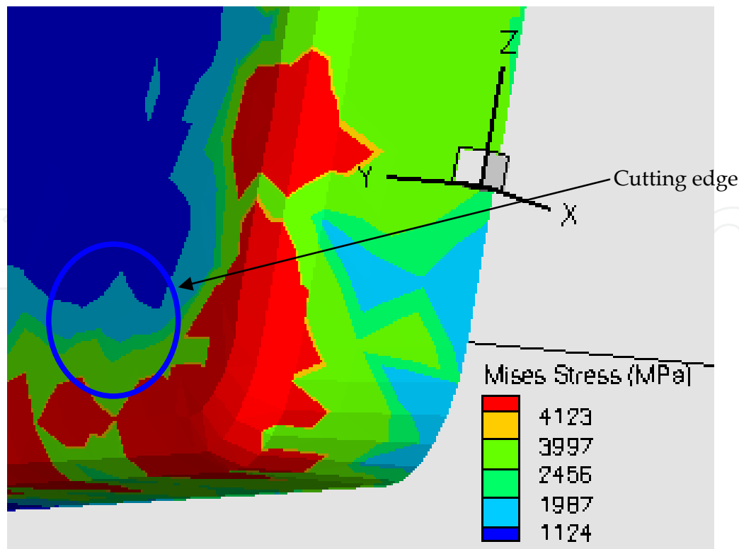
Fig. 6. 3D picture for Von Mises stress distribution for simulation no.9.
