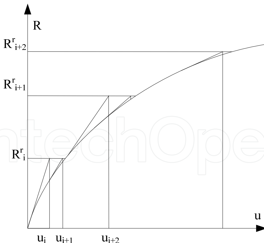
Fig. 6. (a) Modified Newton-Raphson Method
