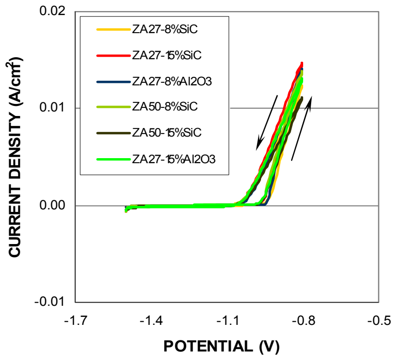
Fig. 2. Voltammograms of (a) pure Zinc with equiaxed structure, (b) pure Zinc with columnar structure (c) Zn-27wt%Al alloy with columnar and equiaxed structures, (d) Zn-27wt%Al alloy with CET structure, (e) pure Aluminum with columnar and equiaxed structure, (f) Zn-27wt%Al + 8vol%SiC, Zn-27wt%Al + 15vol%SiC, (g) Zn-50wt%Al + 8vol%SiC, Zn-50wt%Al + 15vol%SiC, (h) Zn-27wt%Al + 8vol%Al 2 O 3 , Zn-27wt%Al + 15vol%Al 2 O 3 and (i) All types of composites.
