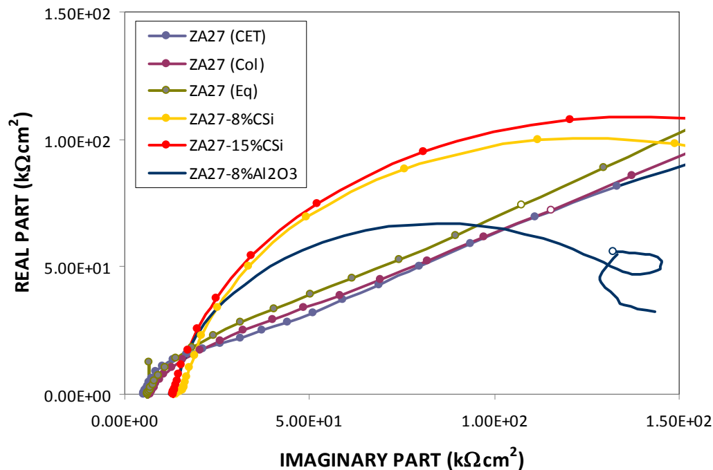
Fig. 6. (a) Nyquist Diagram for different samples.
