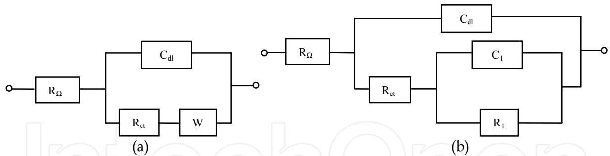
Fig. 8. Equivalent circuit of EIS for different samples.
