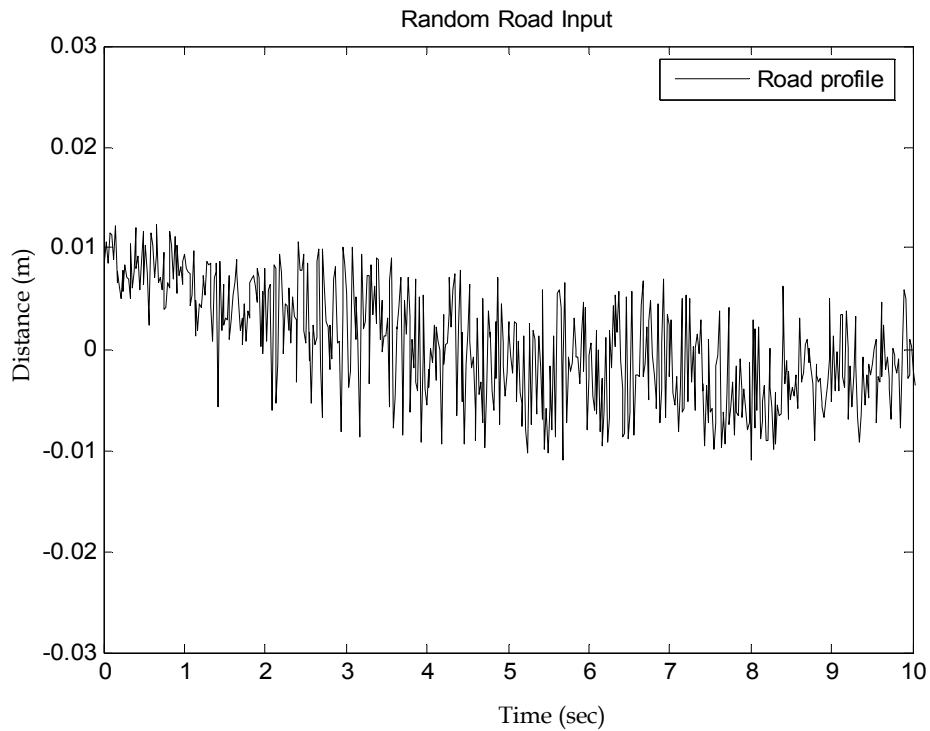
Fig. 28. Road disturbance Vs time (Random)
