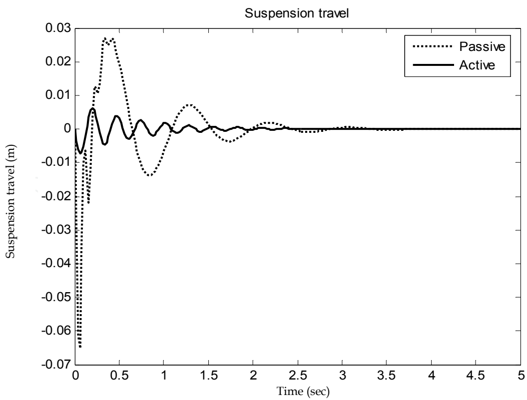
Fig. 25. Suspension travel Vs time (Pot hole)
