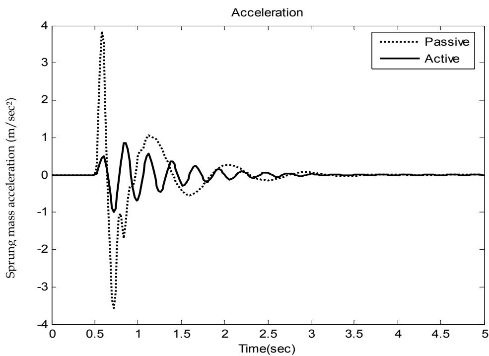
Fig. 20. Sprung mass acceleration Vs time (Bumpy road)
