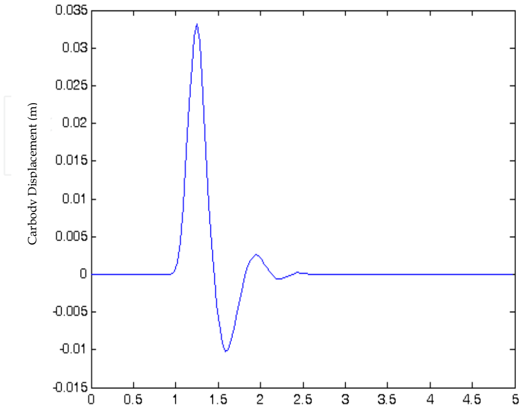
Fig. 14. Car body displacement of active suspension system
