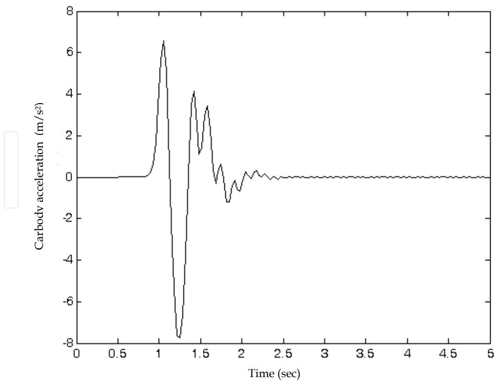
Fig. 15. Car body acceleration of passive suspension system
