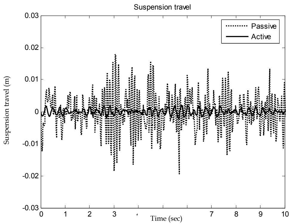
Fig. 31. Suspension travel Vs time (Random road)
