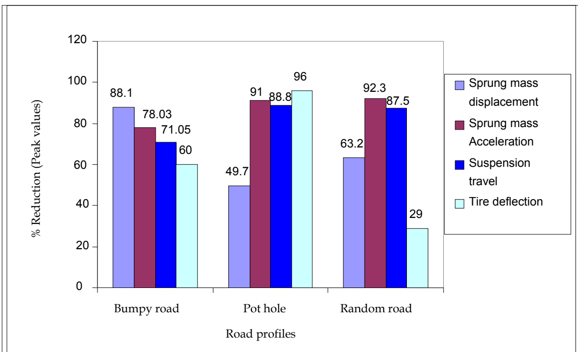
Fig. 33. Active system performance for various road inputs
