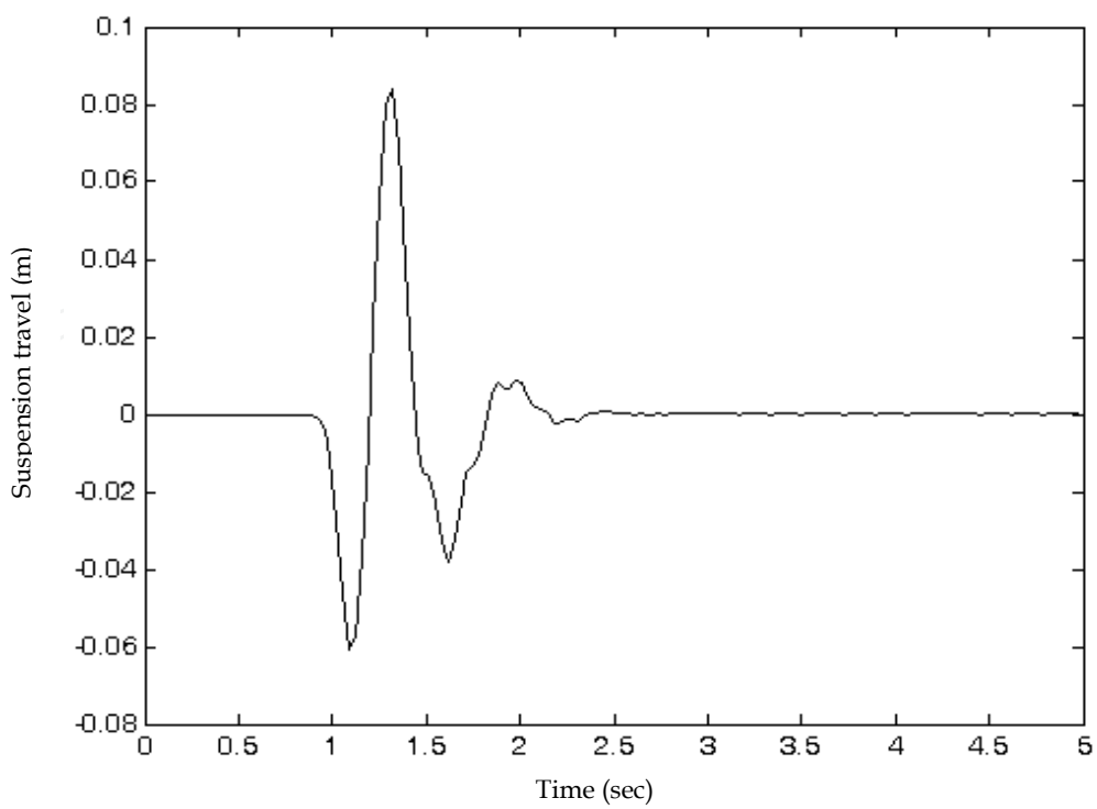
Fig. 17. Suspension travel of passive suspension system
