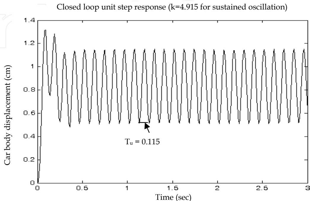
Fig. 10. Closed loop unit step response ( k=4.915 ) for sustained oscillation
