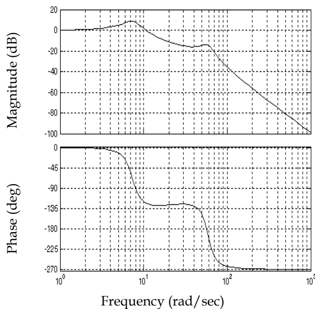
Fig. 7. Bode plot of passive suspension system
