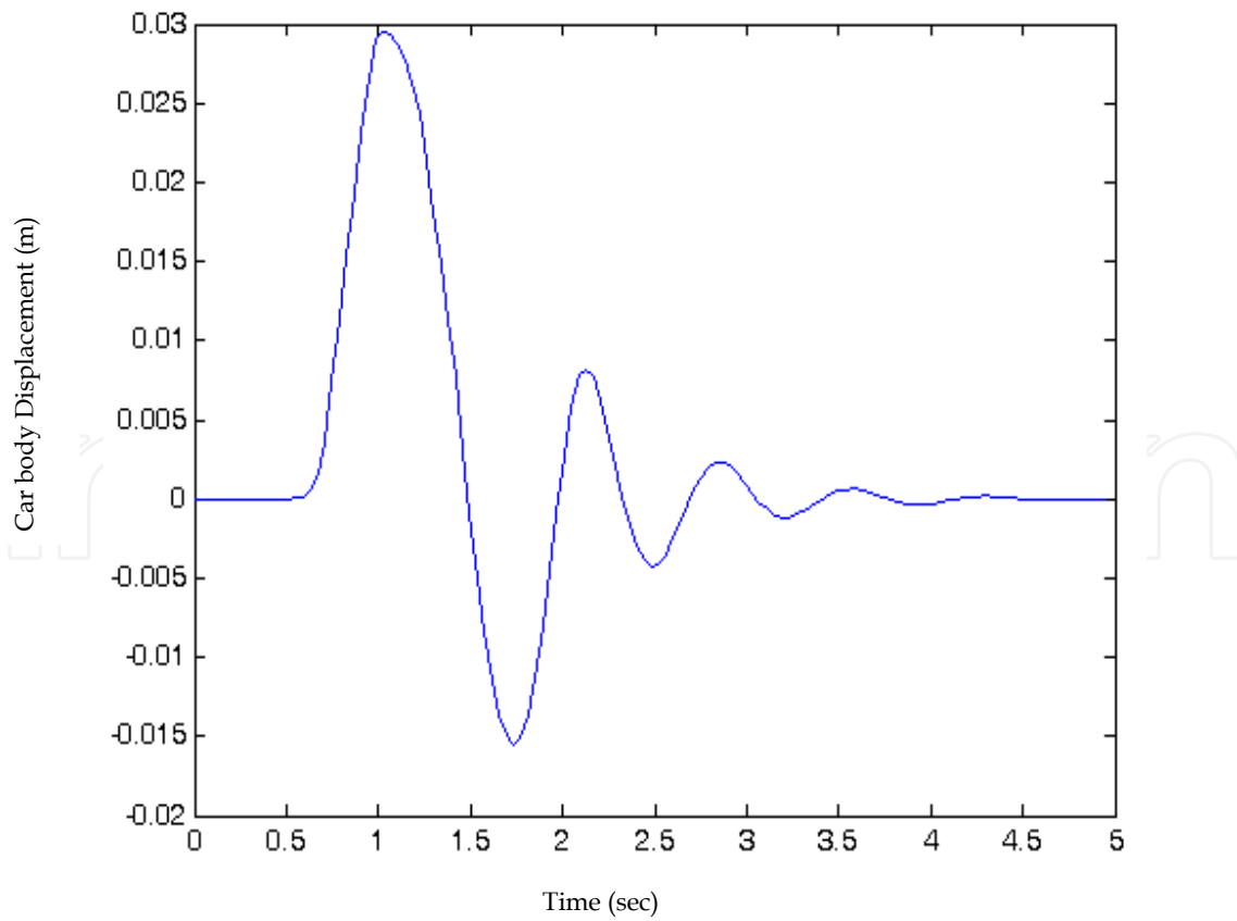
Fig. 13. Car body displacement of passive suspension system
