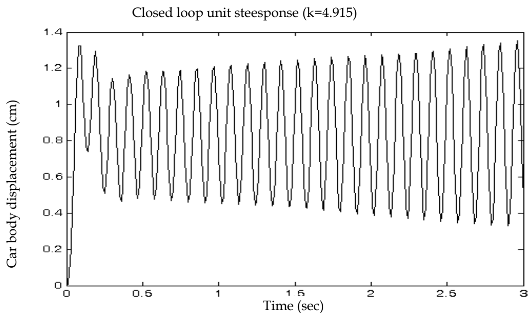
Fig. 9. Closed loop unit step response ( k > 4.915 )
