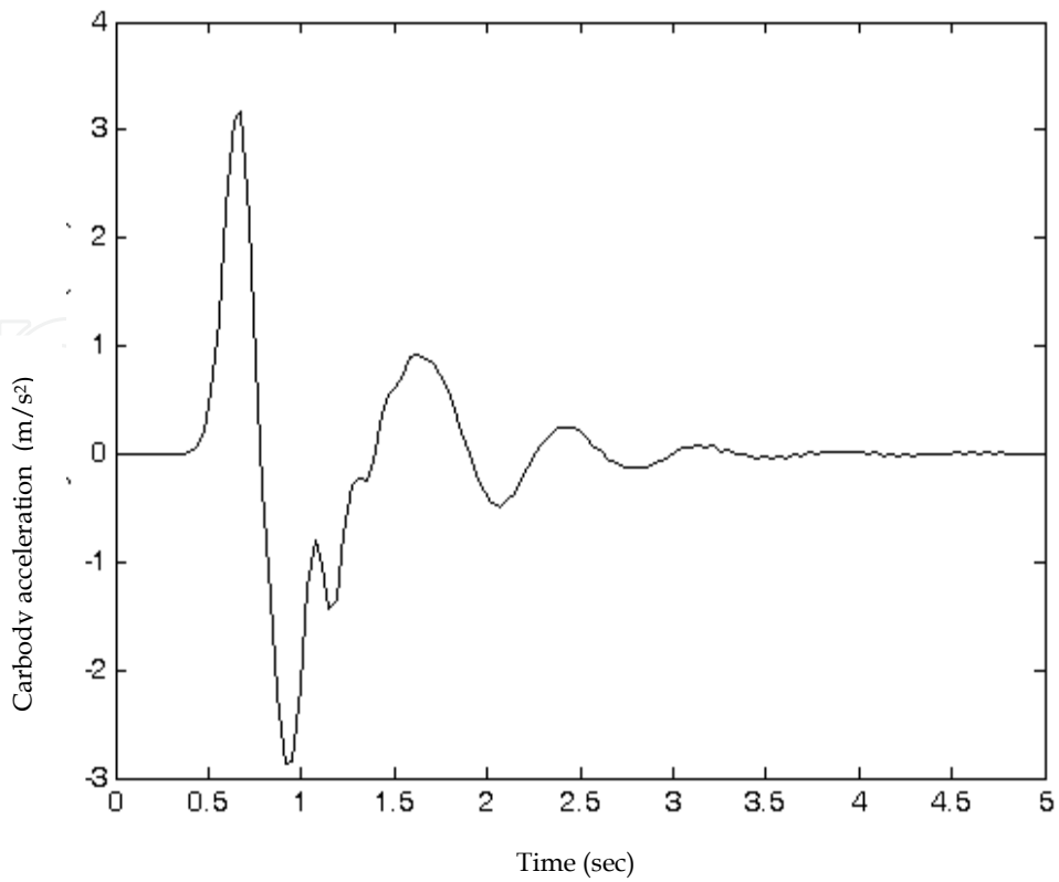
Fig. 16. Car body acceleration of active suspension system
