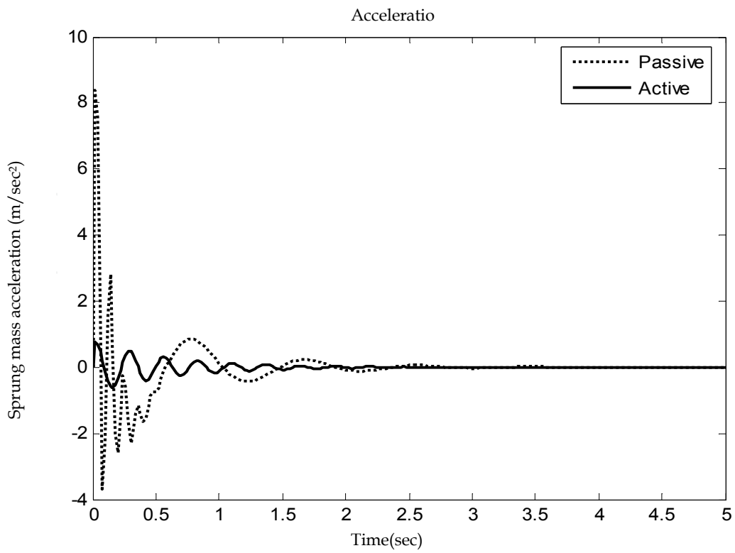
Fig. 24. Sprung mass acceleration Vs time (Pot hole)
