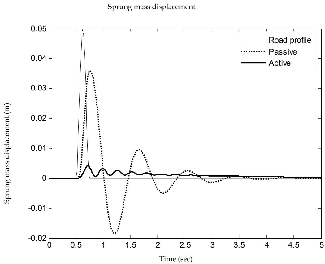
Fig. 19. Sprung mass displacement Vs time (Bumpy road)
