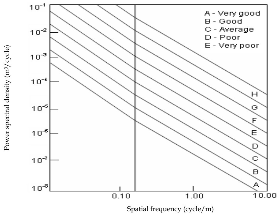
Fig. 27. Road roughness classification by ISO (2000)
