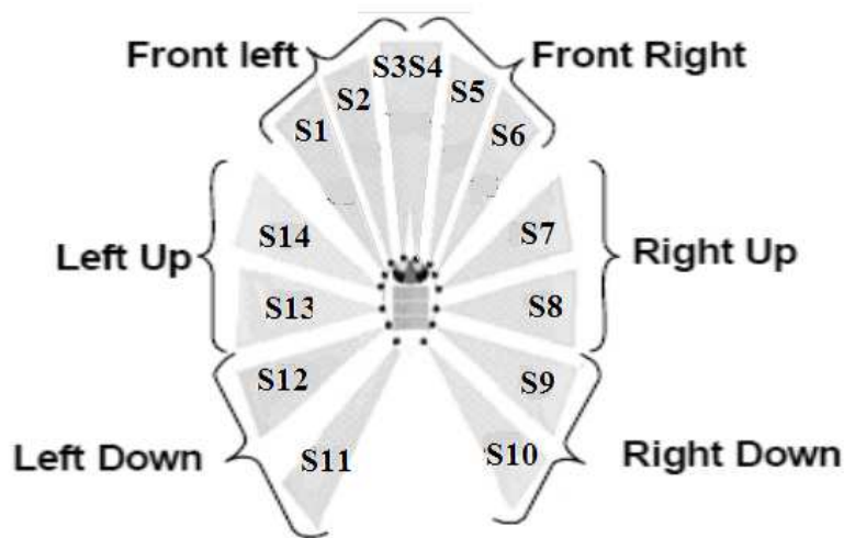
Fig. 8. Infrared sensors arrangement
