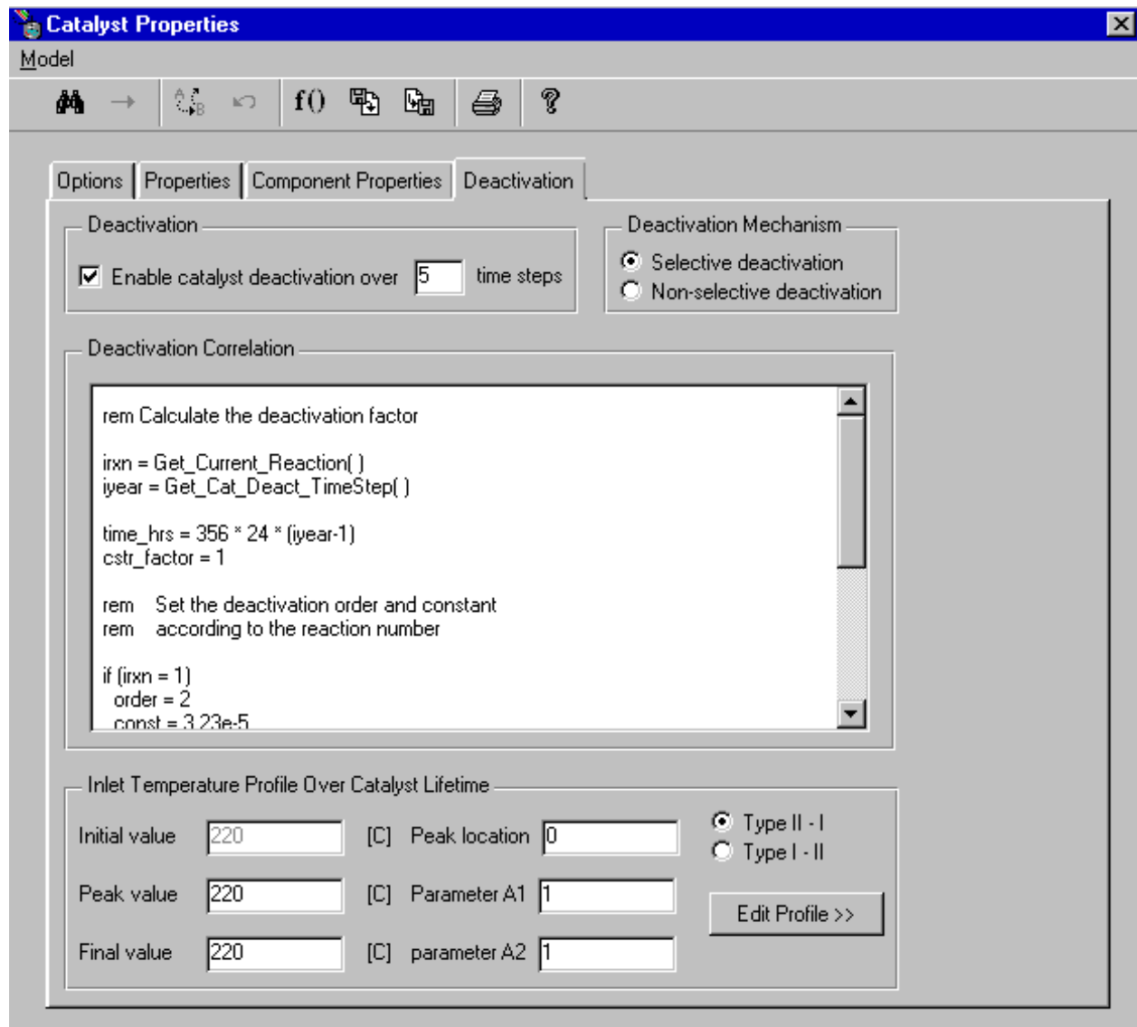
Fig. 4. Catalyst deactivation modeling window in REACTOR
