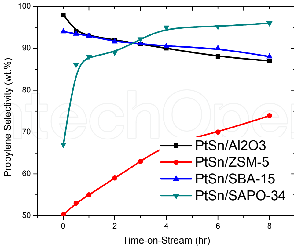
Fig. 8. Catalysts selectivity of propylene over different supported PtSn-based catalysts
