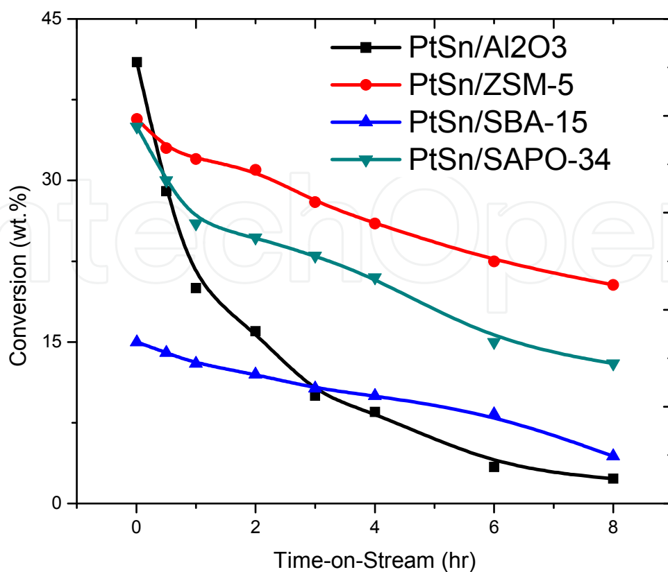
Fig. 7. Catalysts activity at 586 °C for propane conversion
